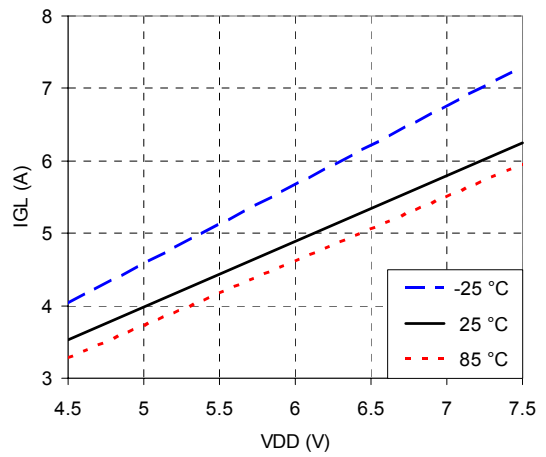
FIGURE 13. LS PULL-DOWN CURRENT WITH TEMPERATURE ( V_{\text{GL}} = 2.5\text{V} , \text{LSEL} = \text{VDD} )
