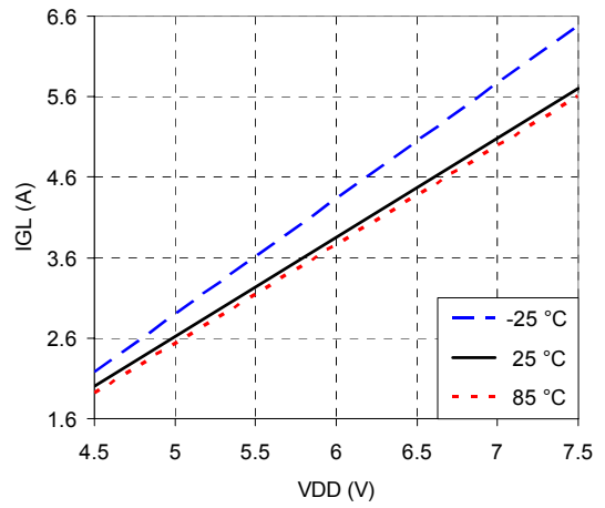
FIGURE 11. LS PULL-UP CURRENT WITH TEMPERATURE ( V_{\text{GL}} = 2.5\text{V} , \text{LSEL} = \text{VDD} )
