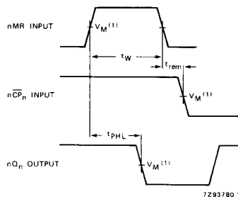
Fig. 7 Waveforms showing the master reset ( nMR ) pulse width, the master reset to output ( nQ_n ) propagation delays and the master reset to clock ( n\overline{CP}_n ) removal time.
