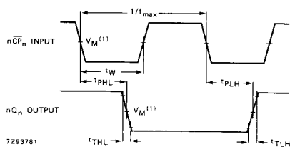
Fig. 6 Waveforms showing the clock ( n\overline{CP}_n ) to output ( nQ_n ) propagation delays, the clock pulse width, the output transition times and the maximum clock frequency.
