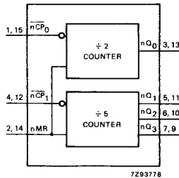
Fig. 4 Functional diagram.
