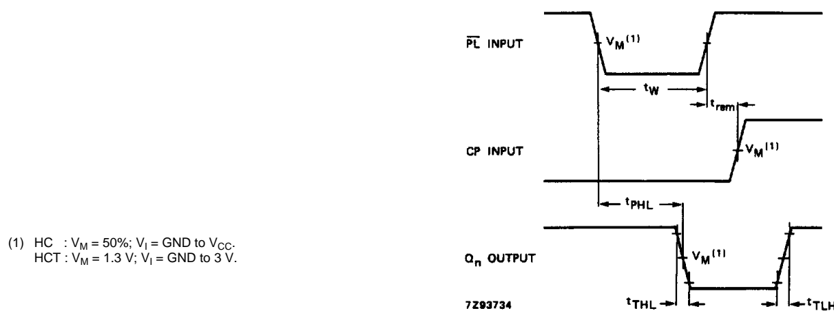
Fig.15 Waveforms showing the parallel load input ( \overline{\text{PL}} ) pulse width, removal time to clock ( \text{CP} ) and the output ( \text{Q}_n ) transition times.
