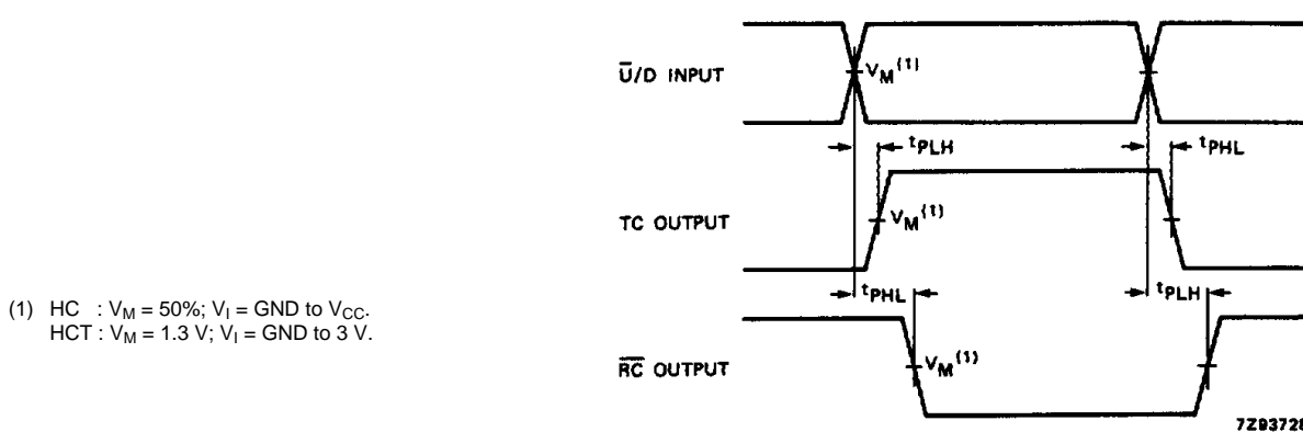
Fig.14 Waveforms showing the up/down count input ( \overline{\text{U/D}} ) to terminal count and ripple clock output ( \text{TC} , \overline{\text{RC}} ) propagation delays.
