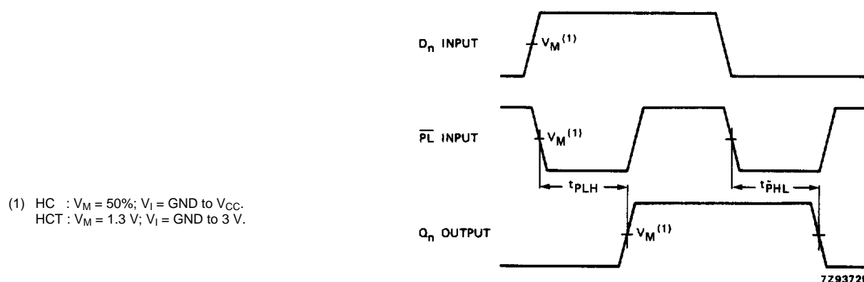
Fig.13 Waveforms showing the input ( \overline{\text{PL}} ) to output ( \text{Q}_n ) propagation delays.
