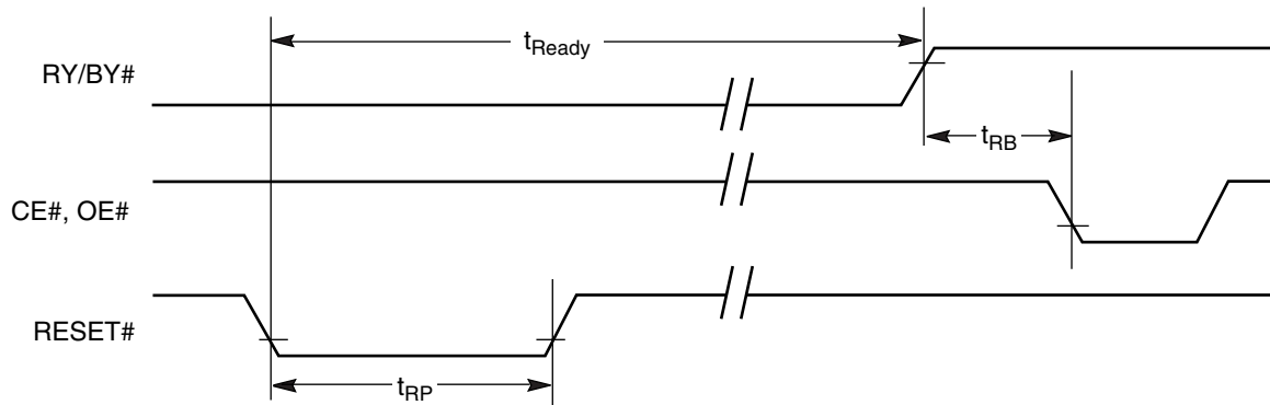
Figure 16. Reset Timings
