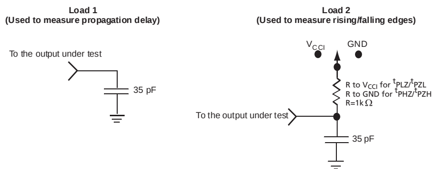
Figure 1-21 • Output Buffer Delays
