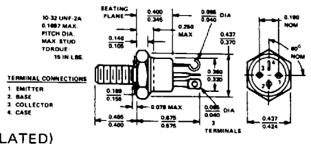
TO-111 (ISOLATED)
