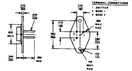
3 PIN TO-66
