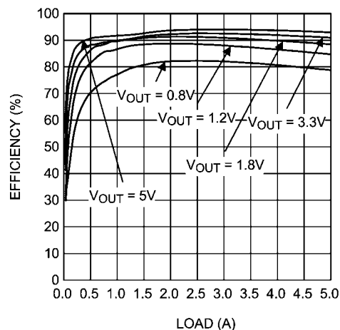
Efficiency with P VIN = 12V, A VIN = 5V, f s = 300 kHz
