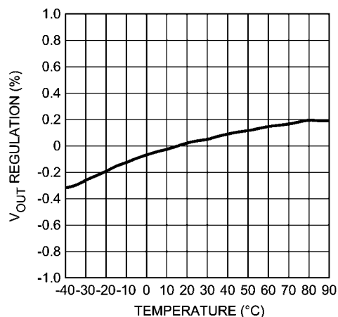
V OUT Regulation (%) vs. Temperature
