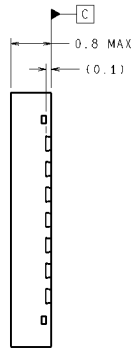
LLP-28 Pin Package NS Package Number SQA28B
