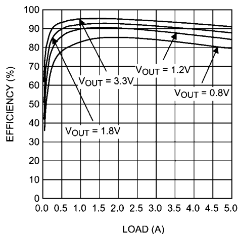
Efficiency with P VIN = A VIN = 5V, f s = 300 kHz
