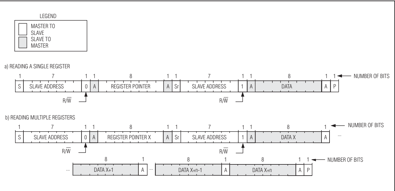
Figures 15a and 15b. Reading from the MAX8649
