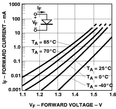
Figure 4. Input Diode Forward Current vs. Forward Voltage.
