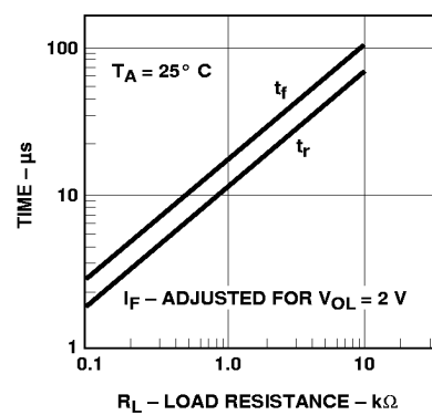
Figure 9. Nonsaturated Rise and Fall Times vs. Load Resistance.
