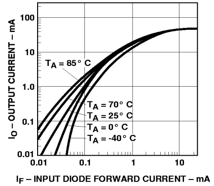
Figure 3. 6N138/6N139 Output Current vs. Input Diode Forward Current.
