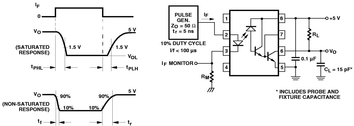
Figure 12. Switching Test Circuit.
