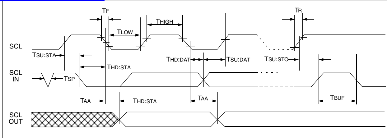
查询"24LC16B-IP"供应商 FIGURE 1-2. BUS TIMING DATA
