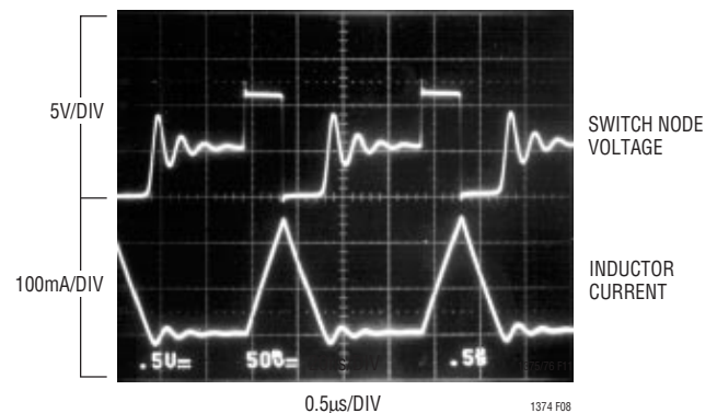
Figure 8. Discontinuous Mode Ringing
