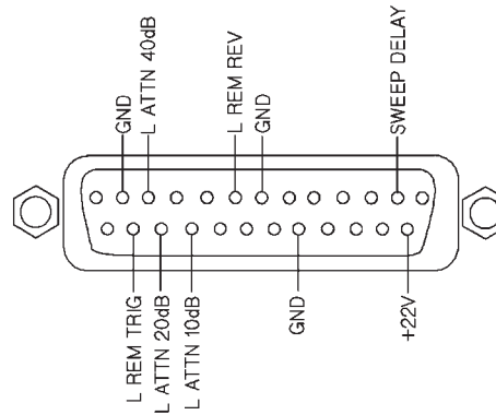
Figure 1-11. S-parameter test set interface pin assignments
