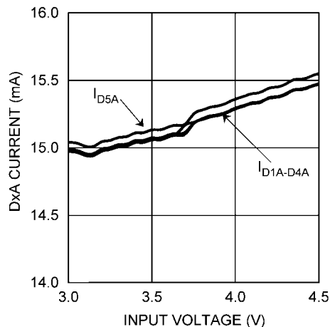
BankA Current Matching vs Input Voltage
