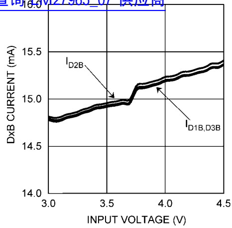
BankB Current Matching vs Input Voltage 查询"LM27965_07"供应商
