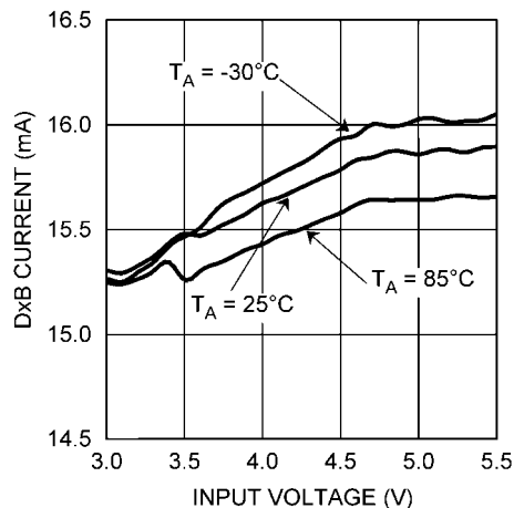
BankB Current Regulation vs Input Voltage
