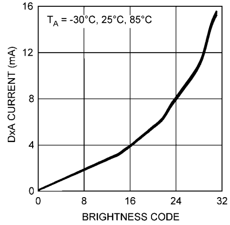
BankA Diode Current vs Brightness Register Code
