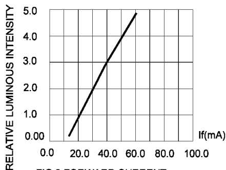
FIG.3 FORWARD CURRENT.
