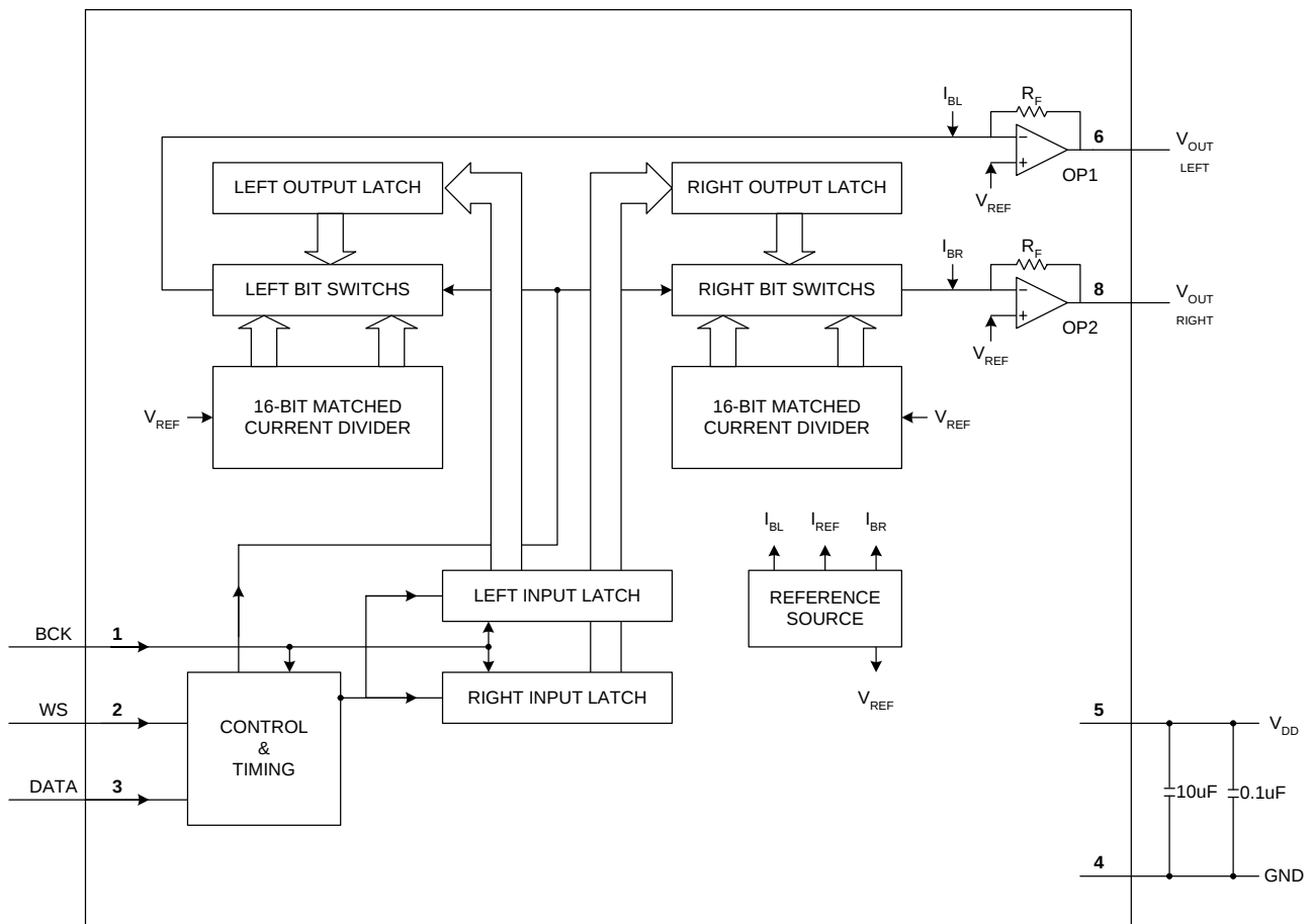
Fig.1 Block diagram.
