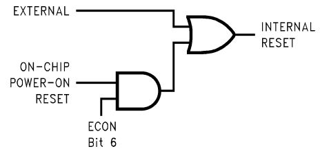
FIGURE 8. Reset Logic
