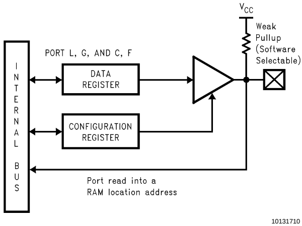
FIGURE 4. I/O Port Configurations
