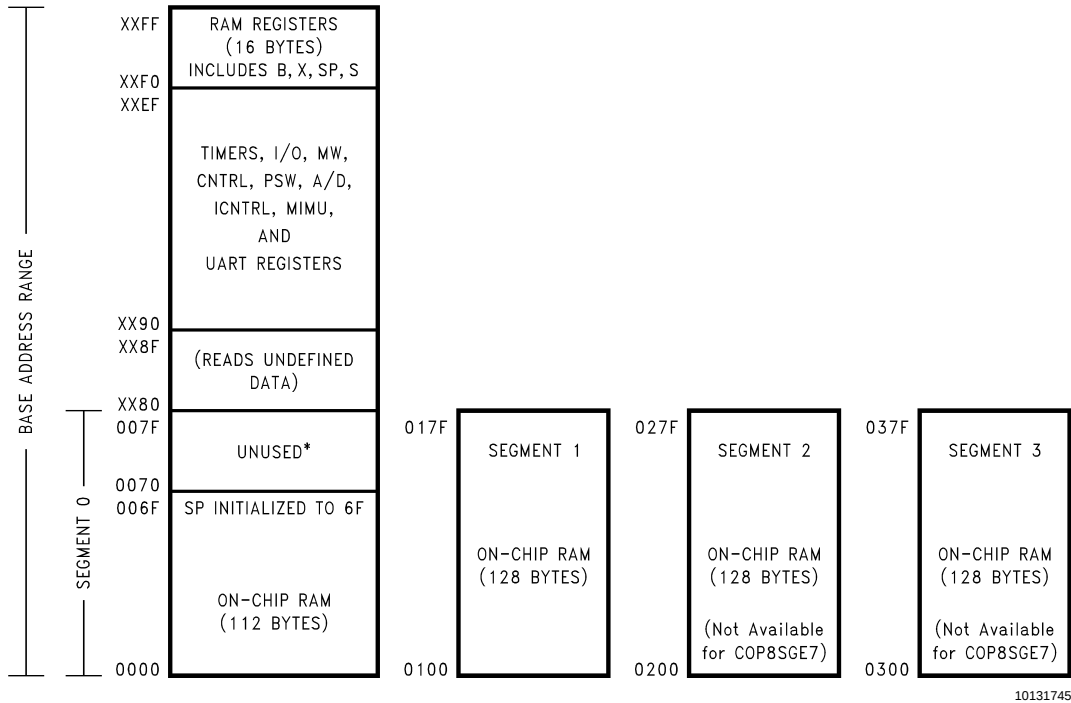
FIGURE 7. RAM Organization
