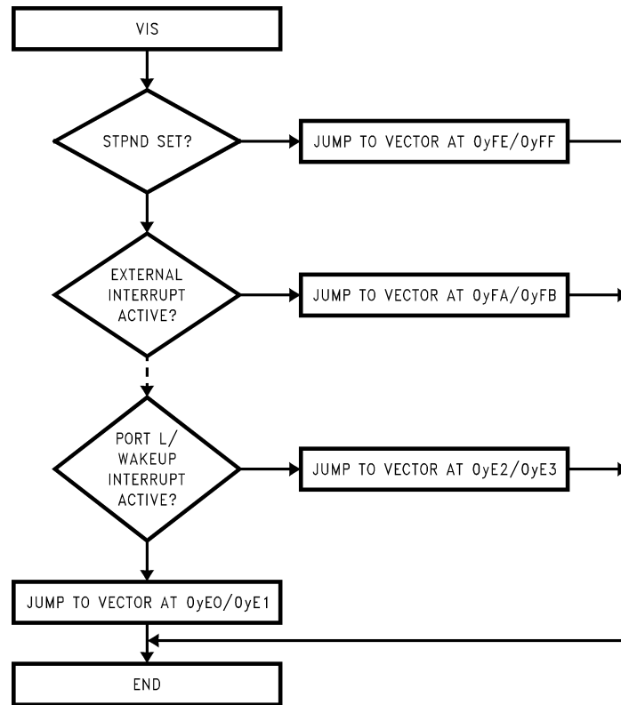
FIGURE 27. VIS Flowchart
