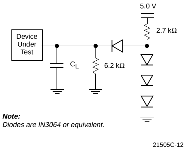
Figure 8. Test Setup
