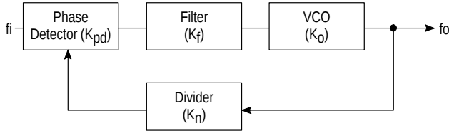
Figure 96. PLL Model
