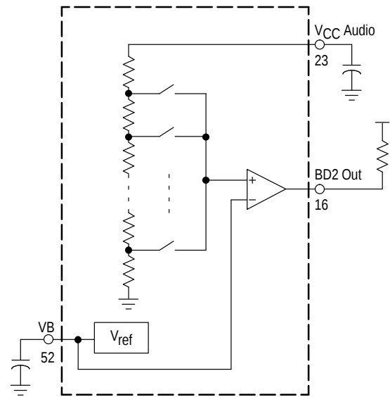
Programmable Threshold Mode: 52-QFP Package
