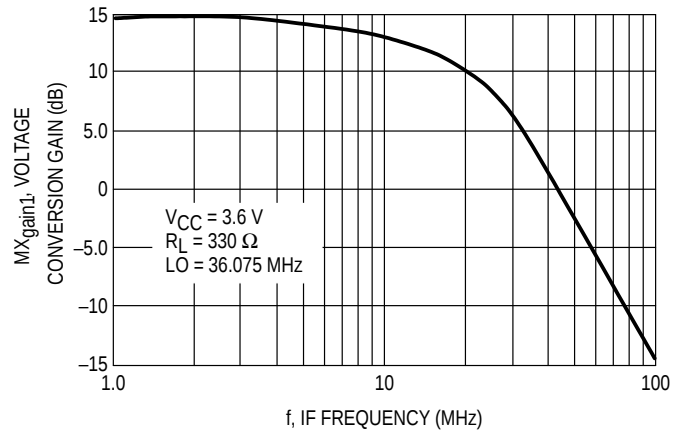
Figure 22. First IF Bandwidth
