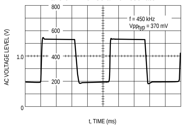
Figure 55. Typical Limiter Output Waveform with Ceramic Resonator
