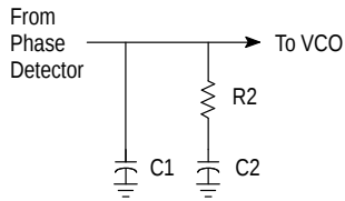
Figure 97. Loop Filter with Additional Integrating Element
