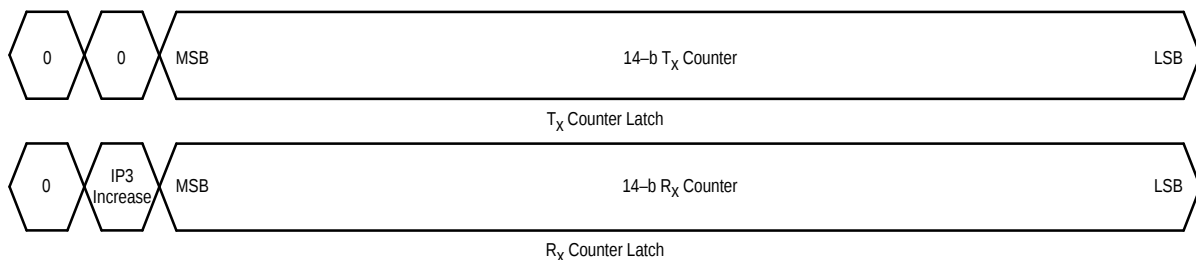
Figure 111. R X and T X Counter Register Latch Bits
