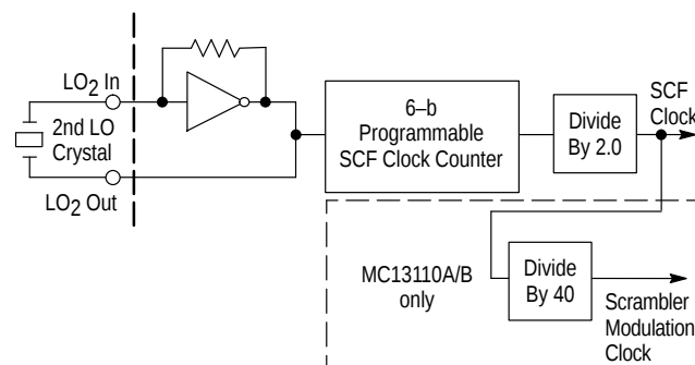
Figure 132. SCF Clock Divider Circuit
