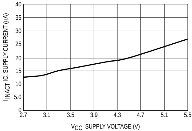
Figure 3. Current versus Supply Voltage Inactive Mode
