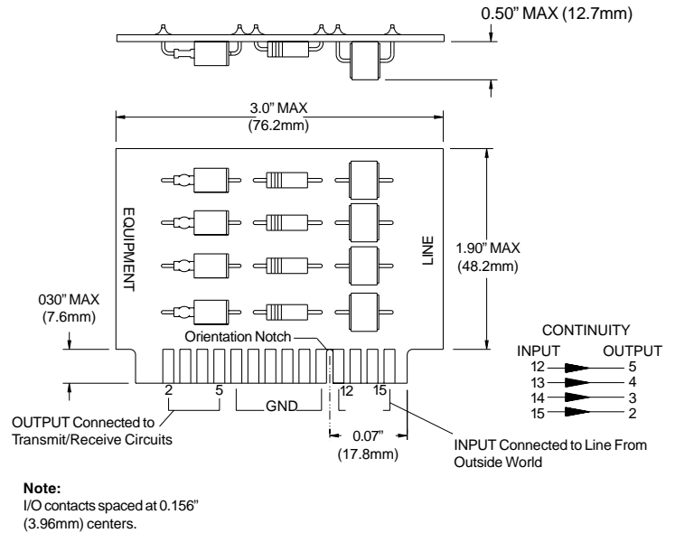
232B Board Outline
