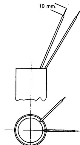
Fig. 5 Cavetti unipolari 0,5mm 2 L = 150 mm Fig. 5 Insulated solid core leads 0.5 mm 2 L = 150 mm
