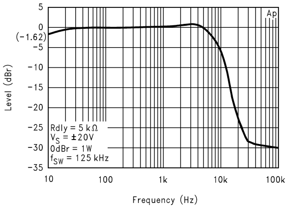
Frequency Response
