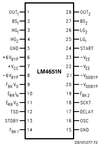
LM4651 Plastic Package
