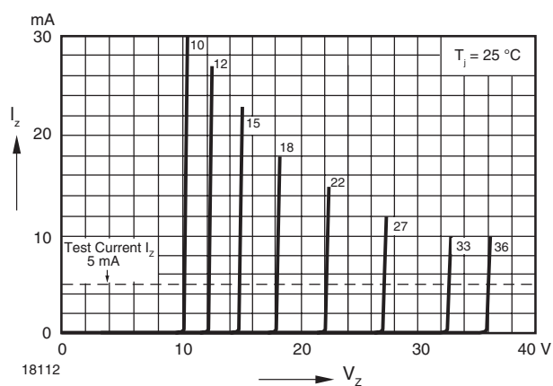
Figure 13. Breakdown Characteristics
