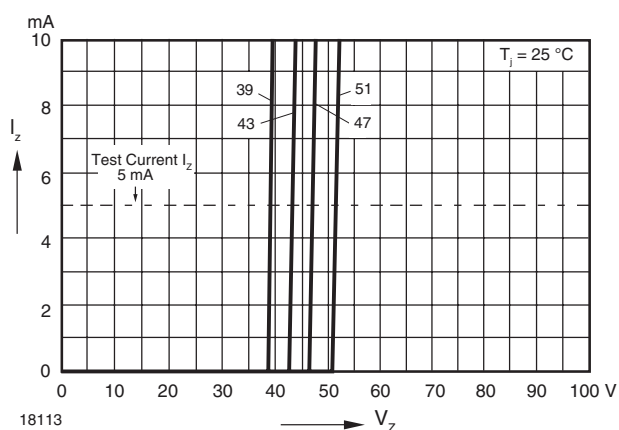
Figure 14. Breakdown Characteristics
