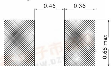
Pad layout
