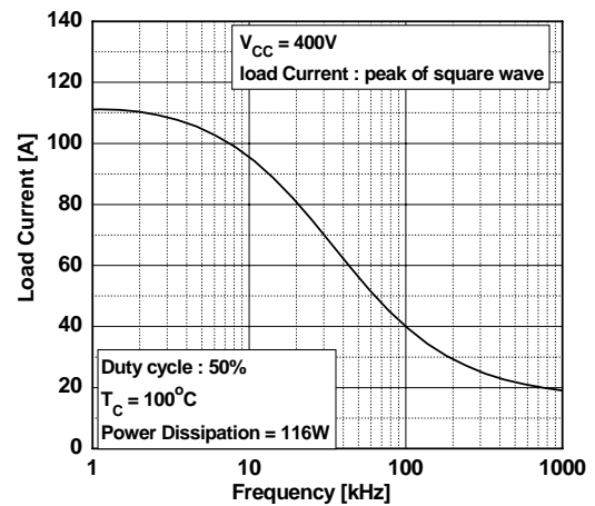
Figure 18. Load Current vs. Frequency
