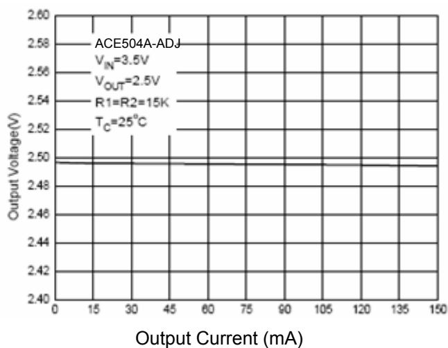
Figure 2. Output Voltage vs. Output Current
