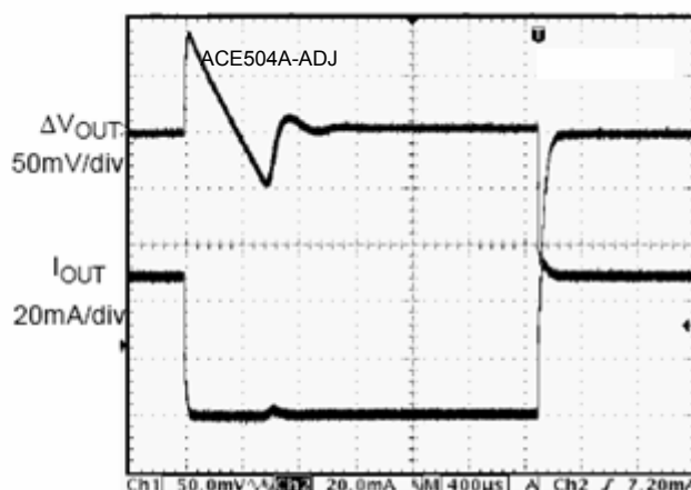
Figure 18. Line Transient
