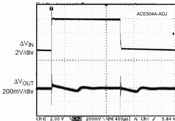
Figure 16. Line Transient (Conditions: V_{IN}=V_{EN}=3.5V to 8V , C_{IN}=1.0\mu F , C_{OUT}=2.2\mu F , I_{OUT}=1mA )
