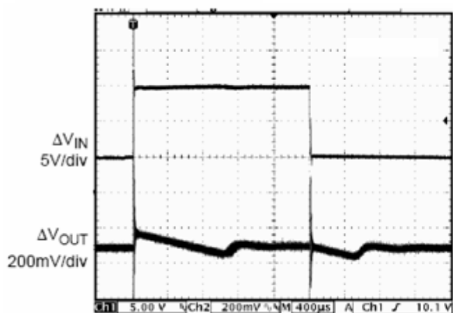
Figure 17. Line Transient
