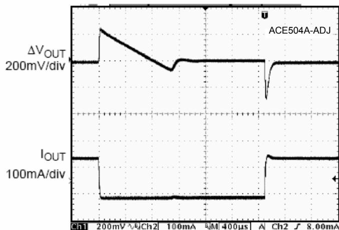
Figure 19. Load Transient
