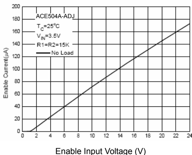
Figure 14. Enable Current vs. Enable Input Voltage
