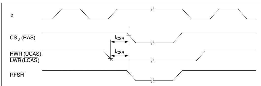
Figure 21.15 DRAM Bus Timing (Self-Refresh Mode) — 2CAS Mode —
