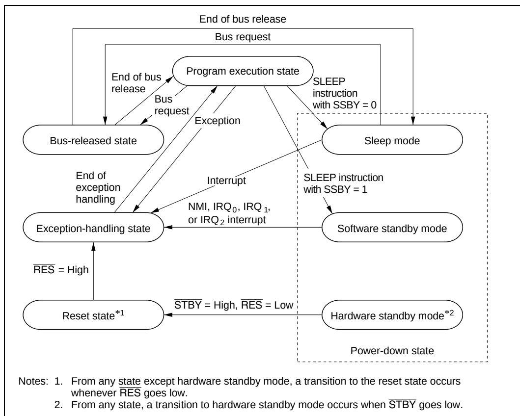
Figure 2.13 State Transitions
