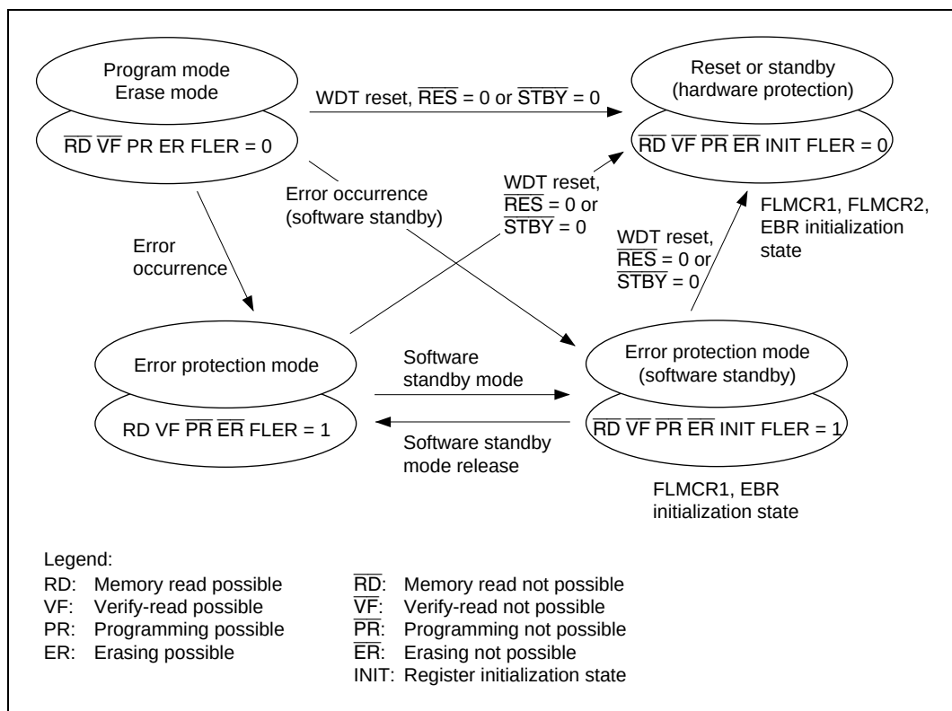
Figure 18.15 Flash Memory State Transitions (When High Level Is Applied to FWE Pin in Mode 5, 6, and 7 (On-Chip ROM Enabled))
