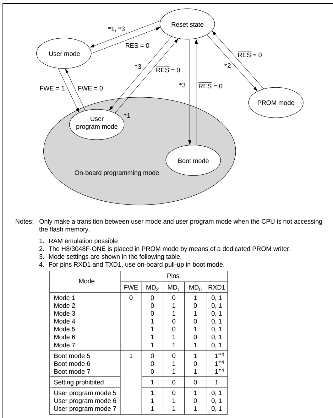
Figure 18.2 Flash Memory State Transitions
