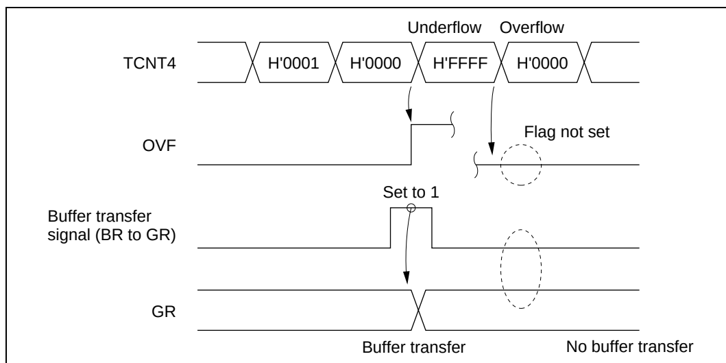
Figure 10.38 Undershoot Timing
