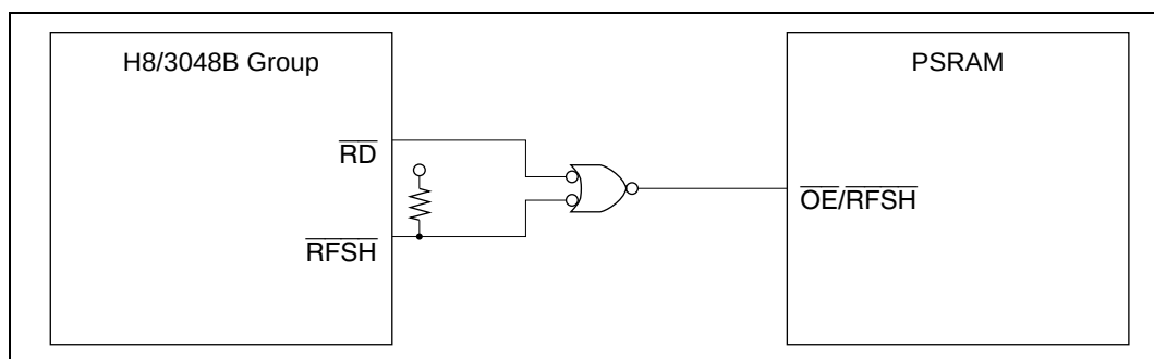
Figure 7.17 Interconnection to Pseudo-Static RAM with \overline{OE/RFSH} Signal (Example)
