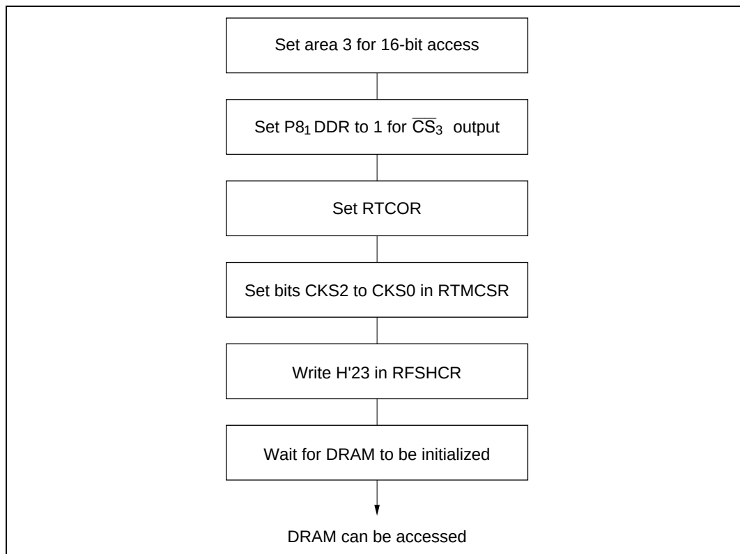
Figure 7.10 Setup Procedure for 2WE 4-Mbit DRAM with 10-Bit Row Address and 8-Bit Column Address (16-Mbyte Mode)
