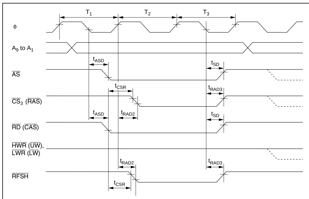
Figure 21.11 DRAM Bus Timing (Refresh Cycle): Three-State Access — 2WE Mode —
