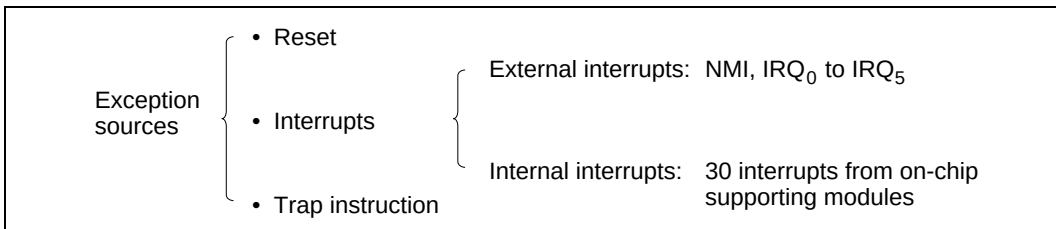
Figure 4.1 Exception Sources
