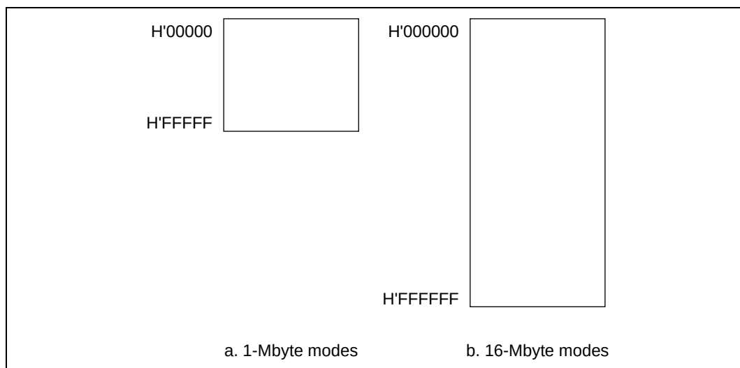
Figure 2.2 Memory Map
