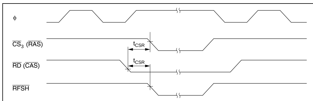
Figure 21.12 DRAM Bus Timing (Self-Refresh Mode) — 2WE Mode —
