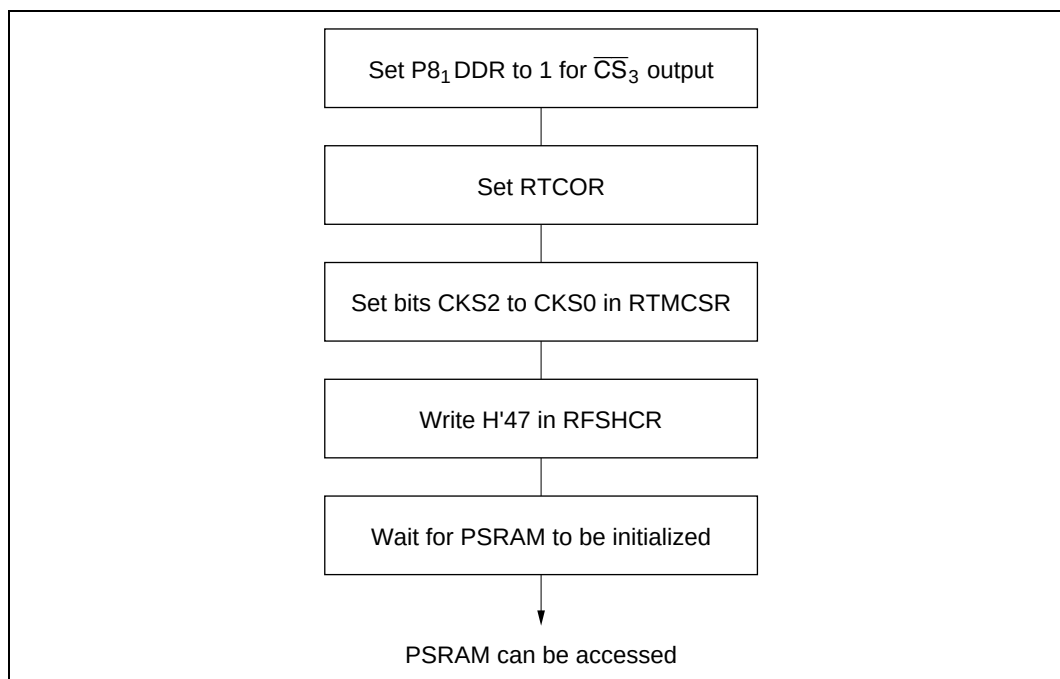
Figure 7.18 Setup Procedure for Pseudo-Static RAM
