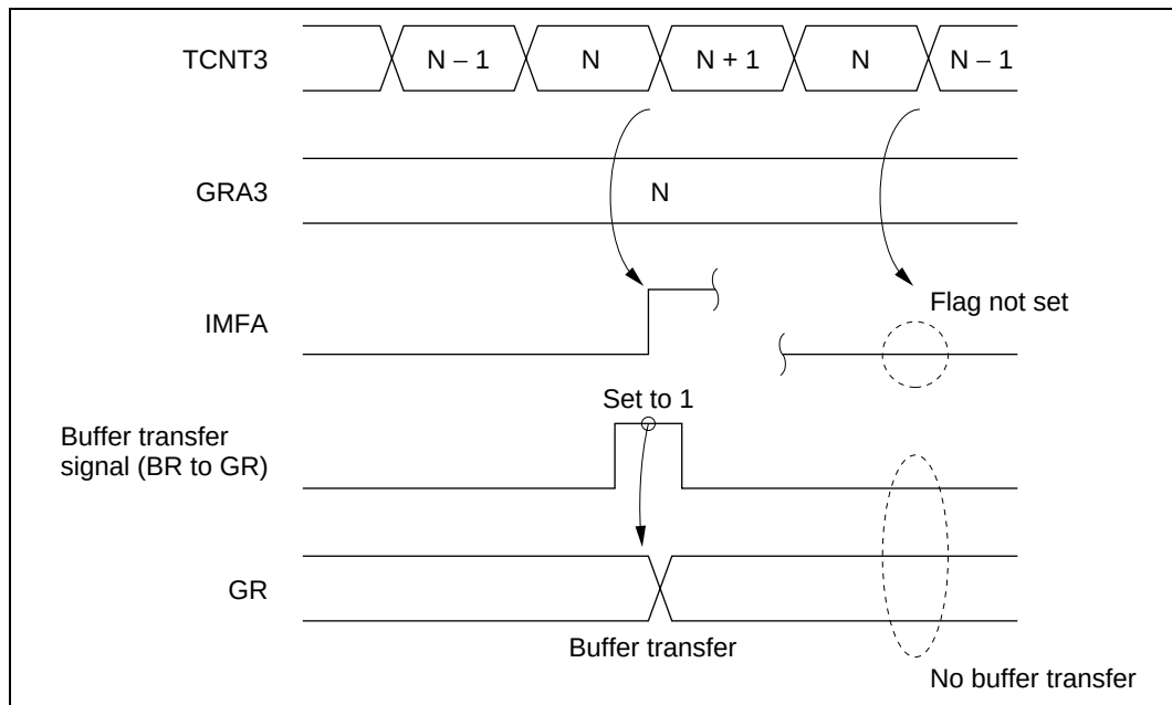
Figure 10.37 Overshoot Timing
