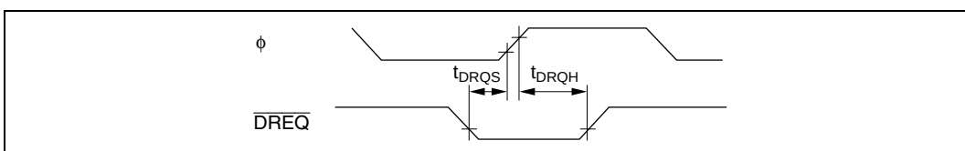
Figure 21.30 DMAC \overline{DREQ} Input Timing
