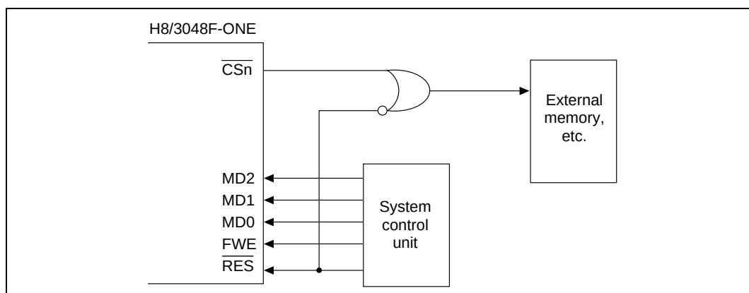
Figure 18.10 Recommended System Block Diagram
