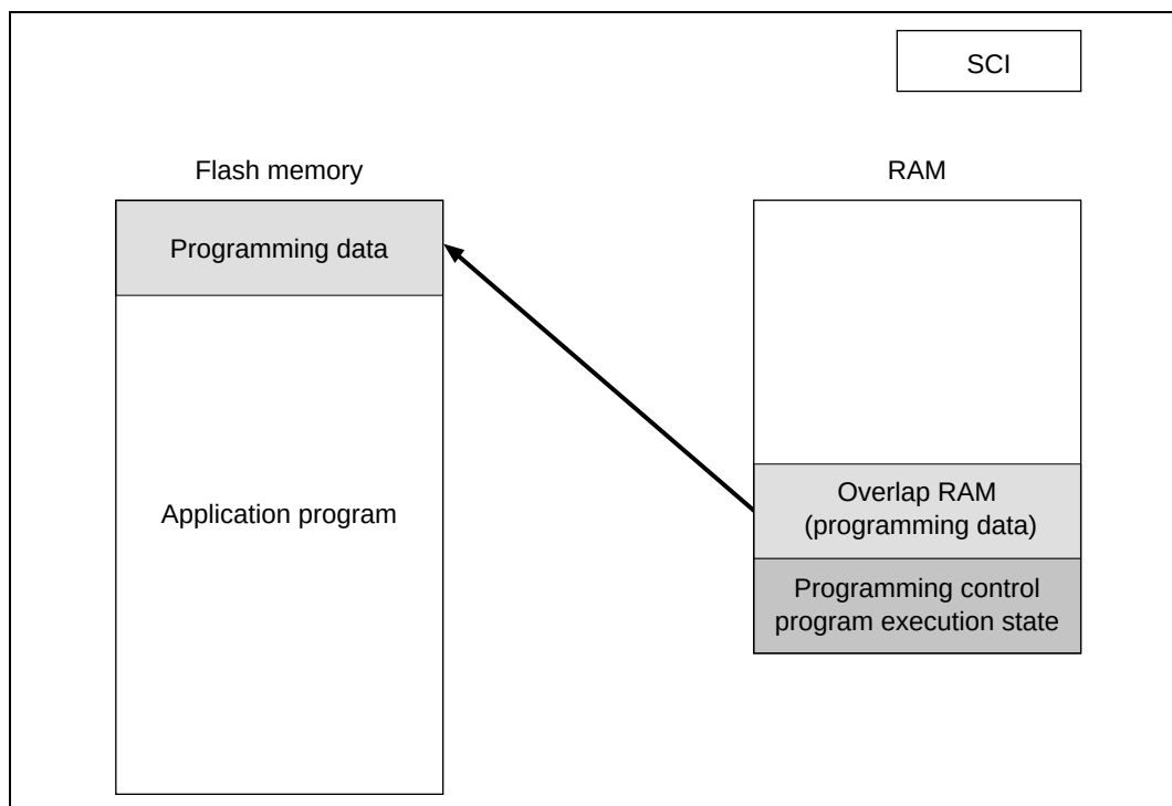
Figure 18.4 Writing Overlap RAM Data in User Program Mode
