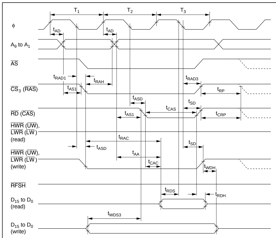
Figure 21.10 DRAM Bus Timing (Read/Write): Three-State Access — 2WE Mode —
