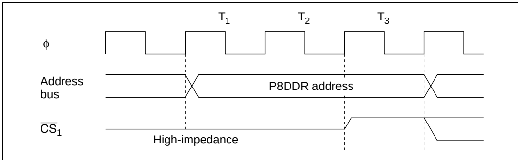
Figure 6.21 DDR Write Timing
