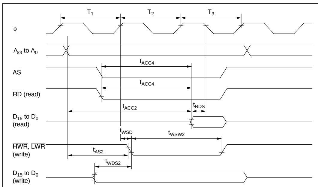
Figure 21.8 Basic Bus Cycle: Three-State Access
