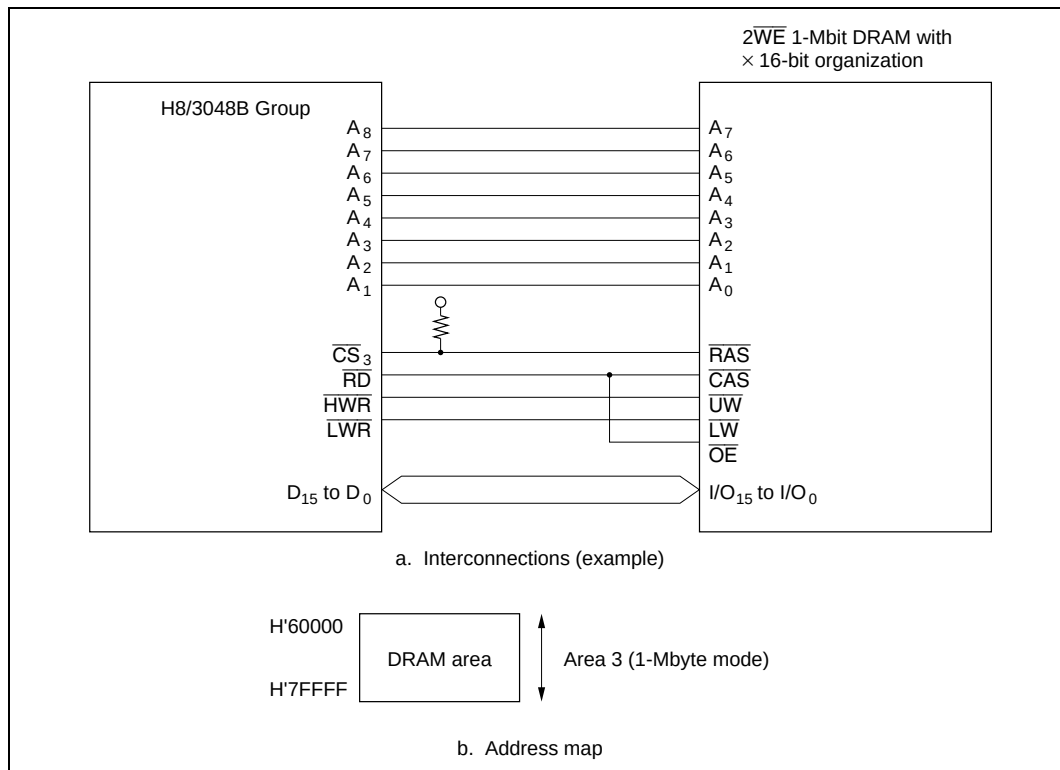
Figure 7.7 Interconnections and Address Map for 2\overline{\text{WE}} 1-Mbit DRAM (Example)
