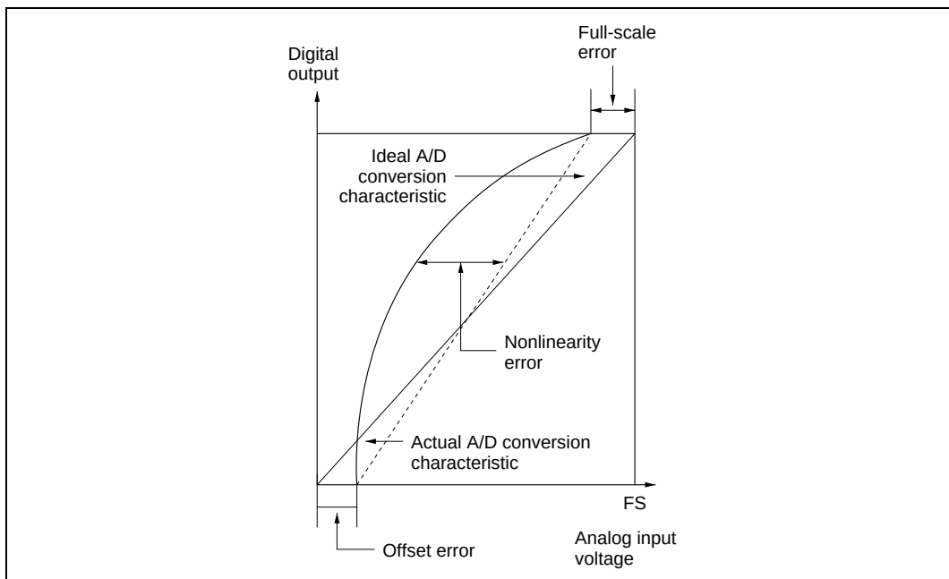
Figure 15.10 A/D Converter Accuracy Definitions (2)
