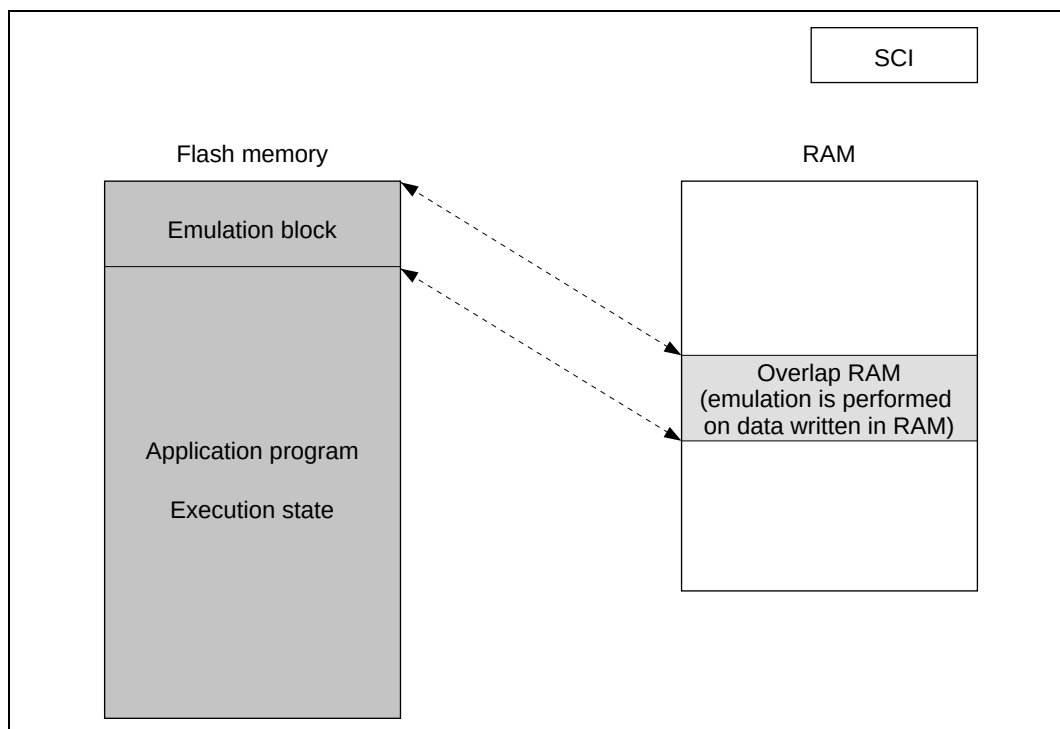
Figure 18.3 Reading Overlap RAM Data in User Mode or User Program Mode
