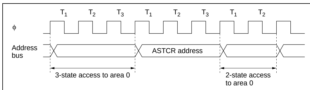
Figure 6.20 ASTCR Write Timing
