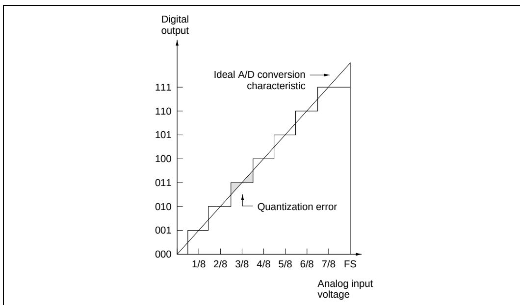
Figure 15.9 A/D Converter Accuracy Definitions (1)
