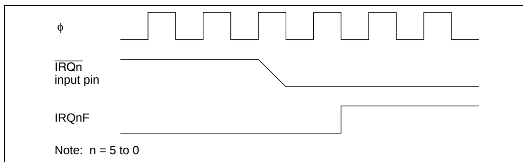
Figure 5.3 Timing of Setting of \text{IRQnF}
