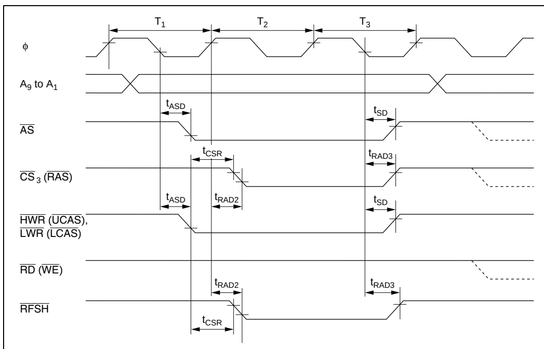
Figure 21.14 DRAM Bus Timing (Refresh Cycle): Three-State Access — 2CAS Mode —
