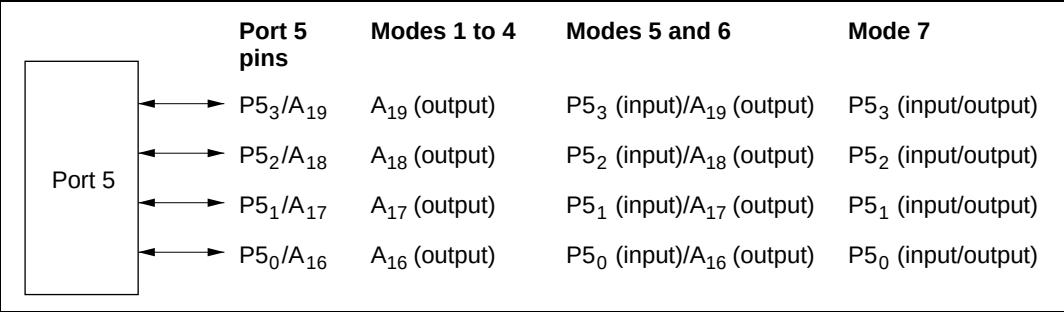
Figure 9.5 Port 5 Pin Configuration
