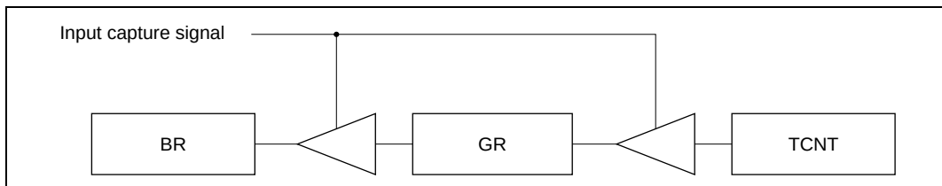
Figure 10.47 Input Capture Buffering
