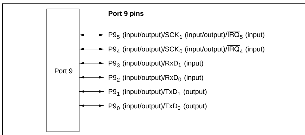
Figure 9.9 Port 9 Pin Configuration
