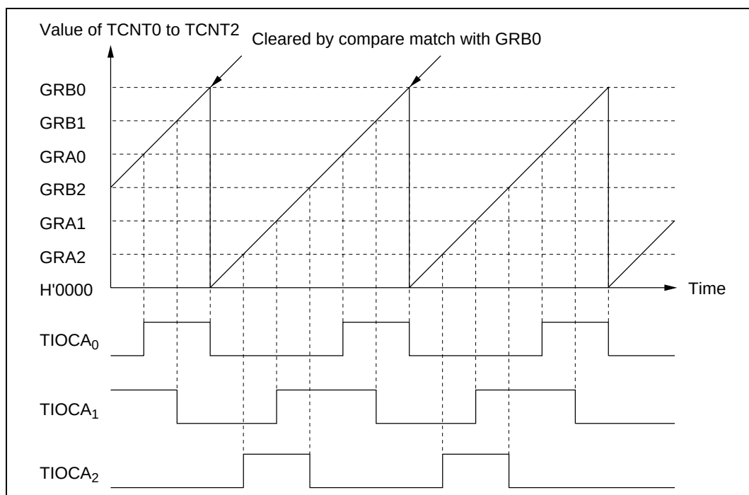
Figure 10.27 Synchronization (Example)
