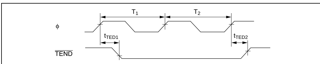
Figure 21.28 DMAC \overline{TEND} Output Timing for 2 State Access
