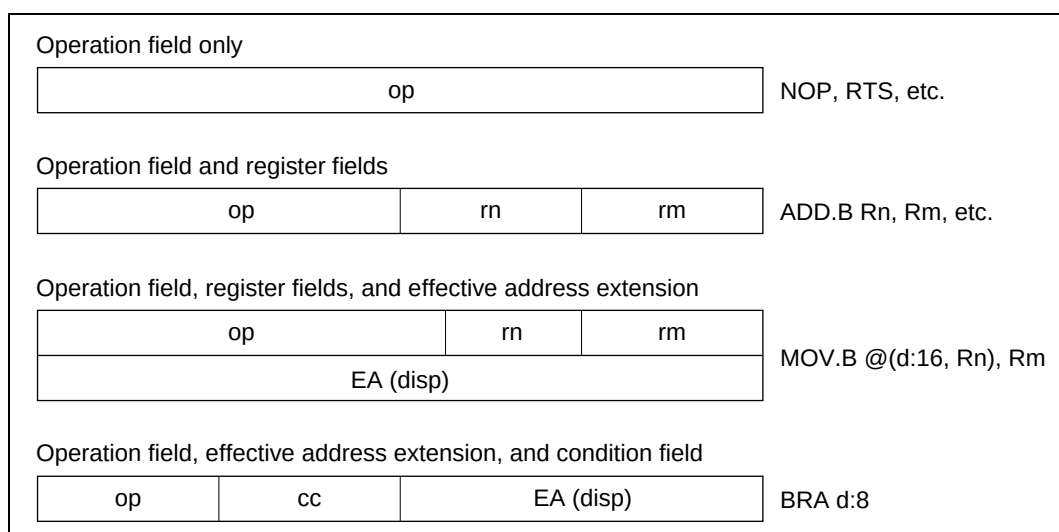
Figure 2.9 Instruction Formats
