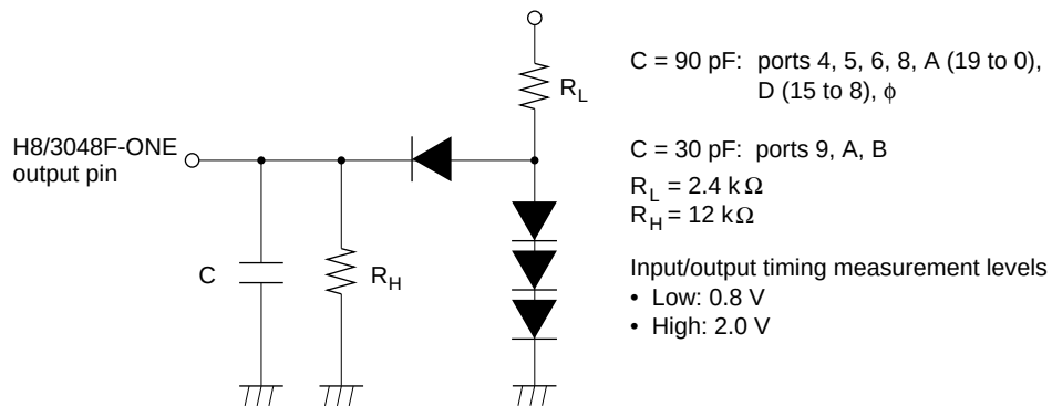
Figure 21.3 Output Load Circuit
