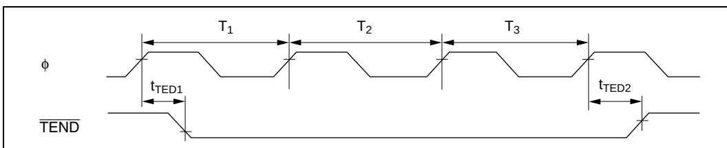
Figure 21.29 DMAC \overline{TEND} Output Timing for 3 State Access
