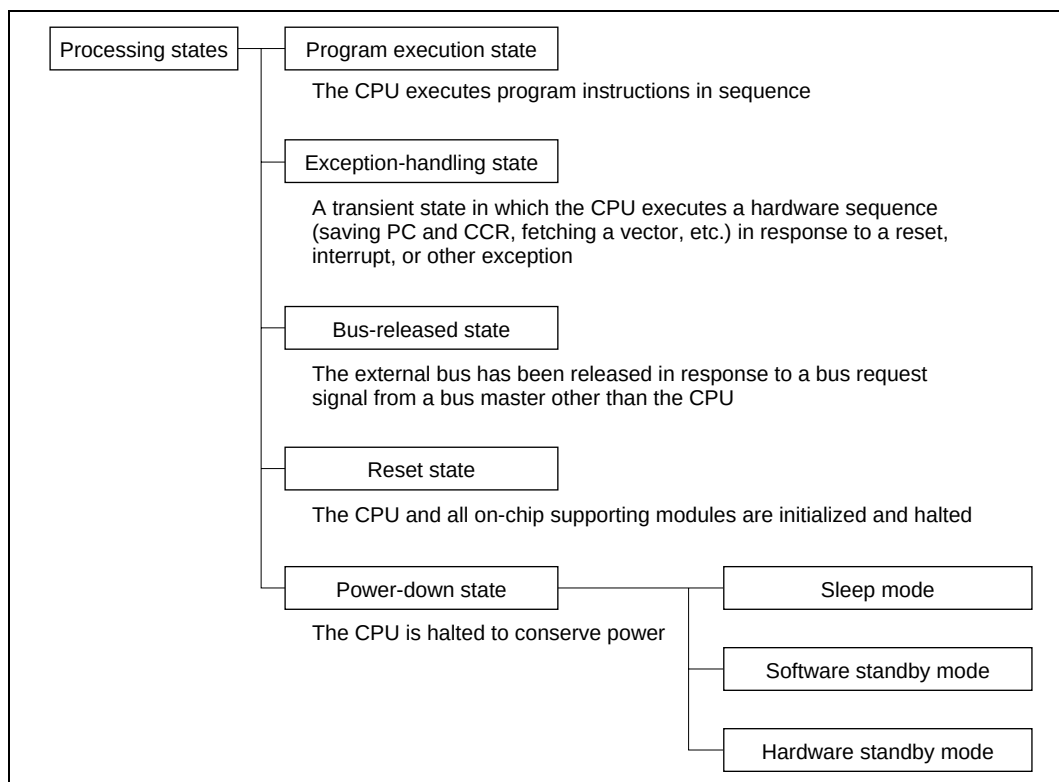
Figure 2.11 Processing States
