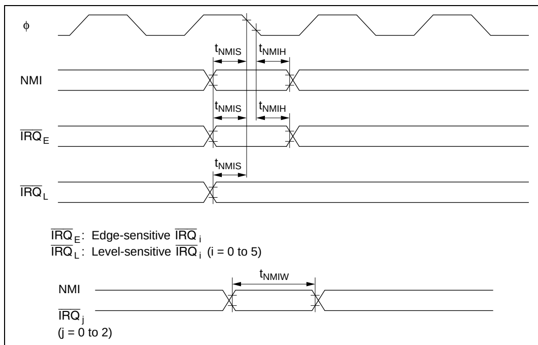
Figure 21.20 Interrupt Input Timing
