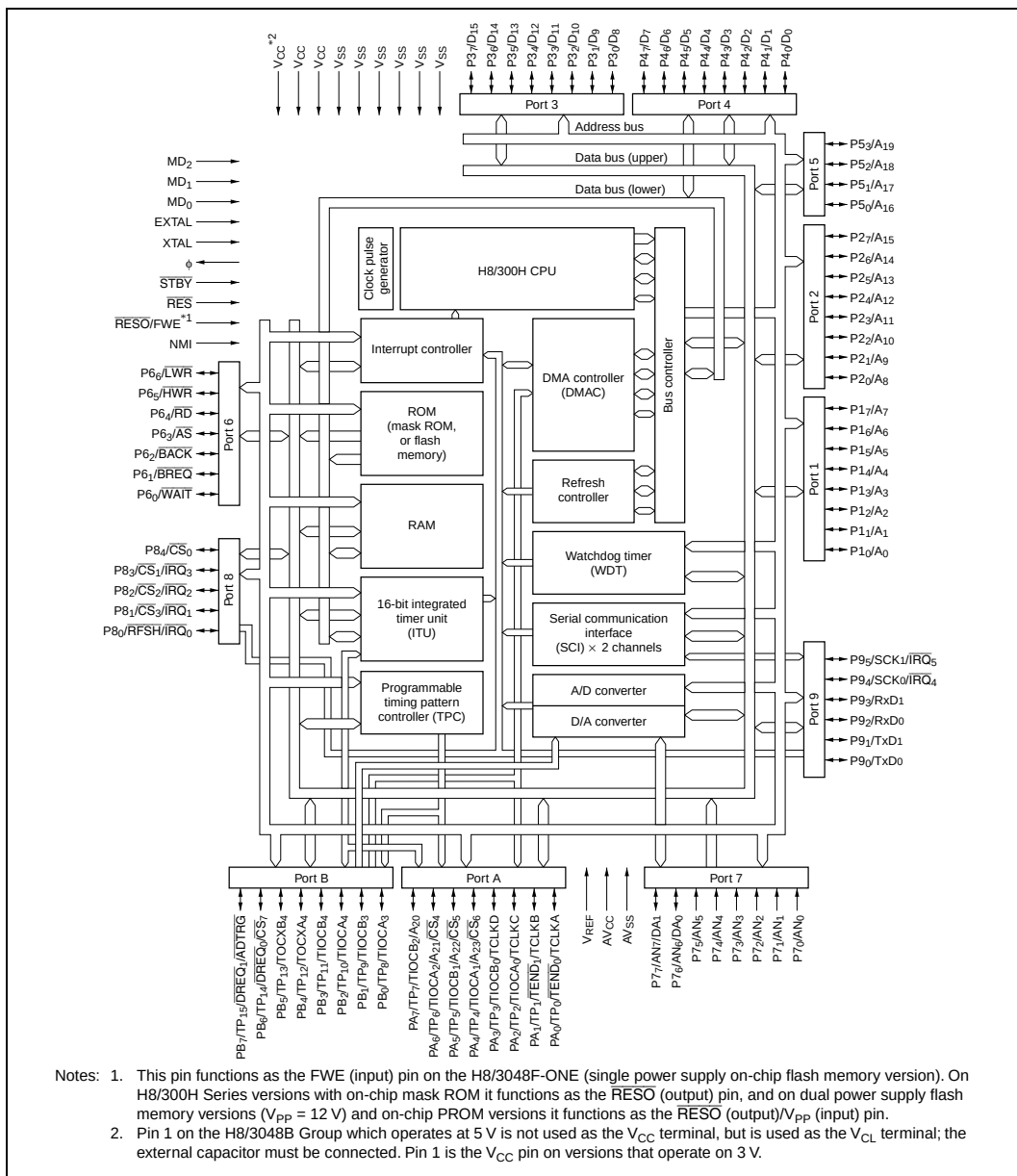
Figure 1.1 Block Diagram
