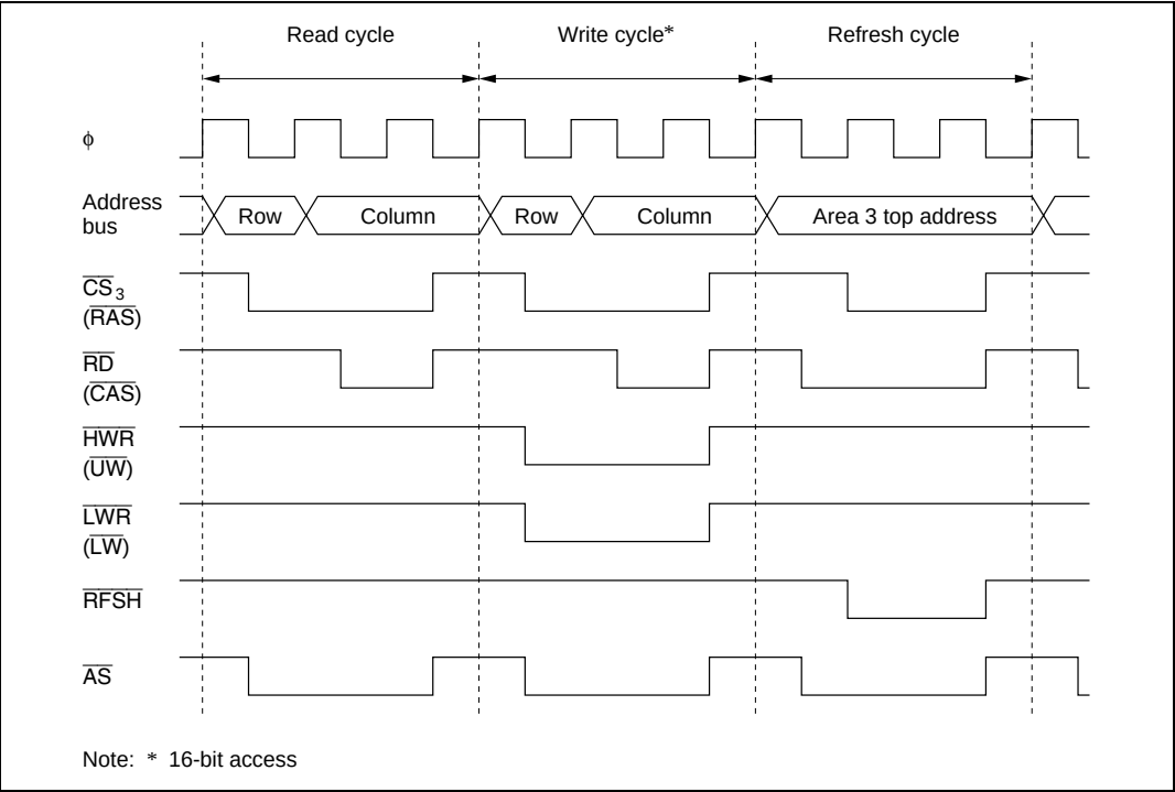
Figure 7.5(1) DRAM Control Signal Output Timing (2WE Mode)
