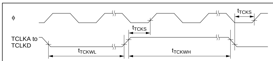
Figure 21.25 ITU External Clock Input Timing
