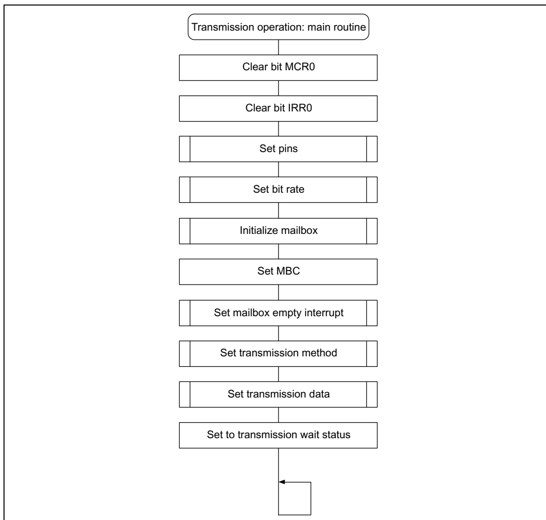
Figure 3.1 Transmission Flowchart (1)
