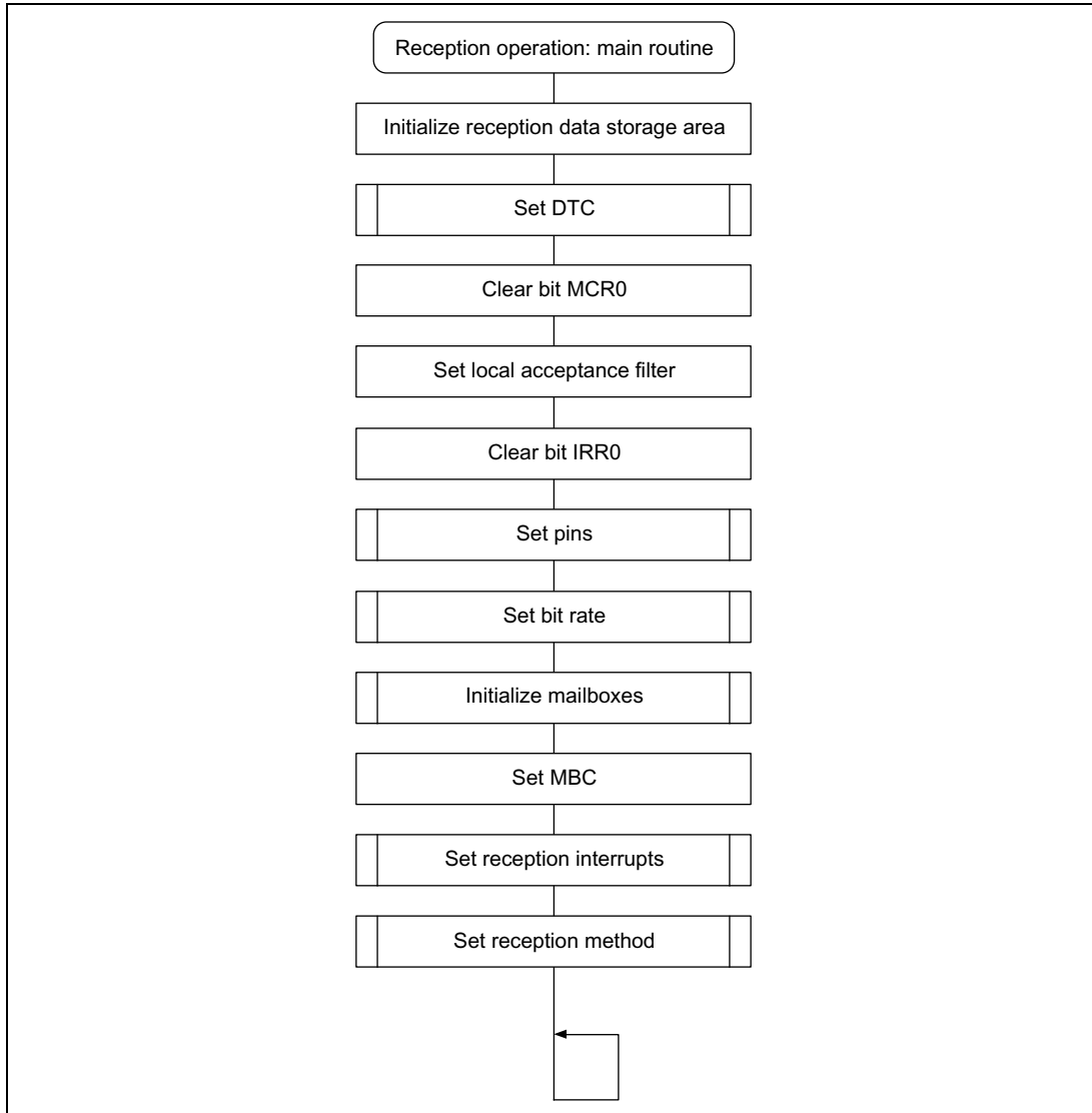
Figure 4.3 Reception Flowchart (1)
