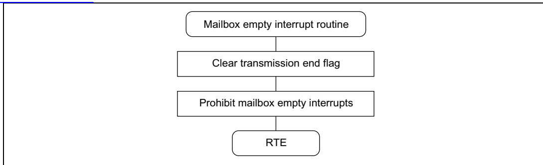
Figure 3.1 Transmission Flowchart (2)
