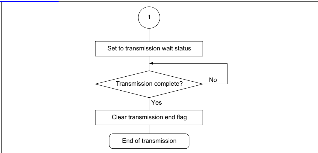
Figure 4.2 Transmission Flowchart (2)
