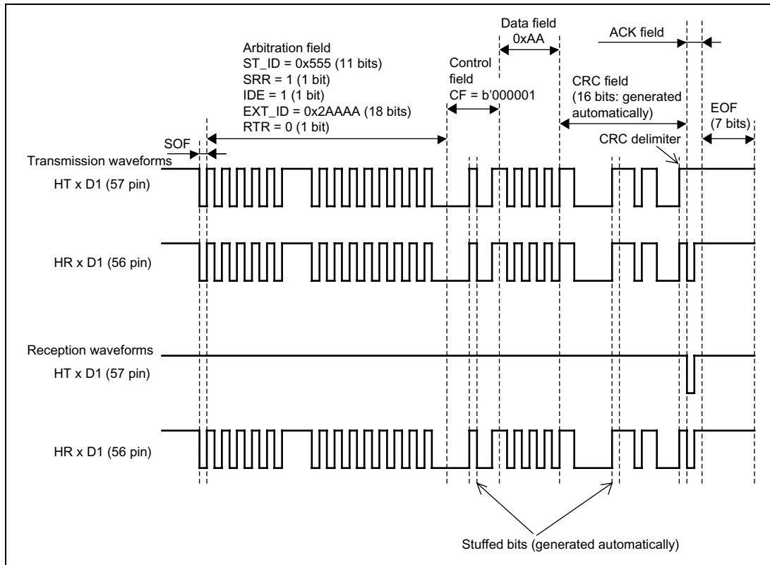
Figure 3.5 Operation Waveforms
