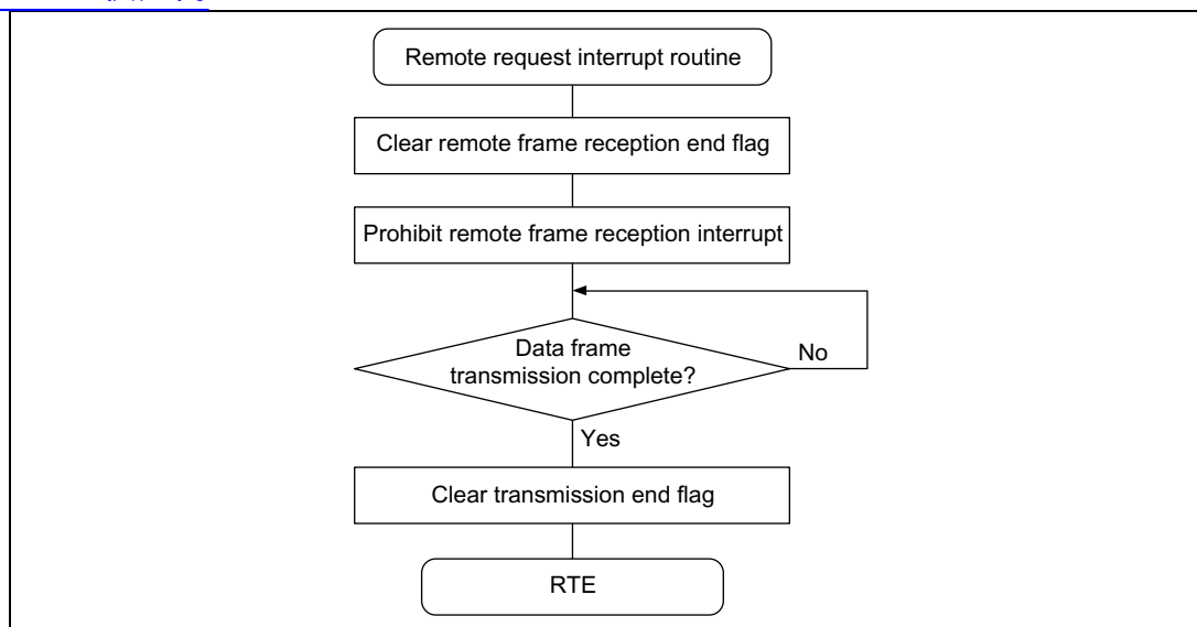
Figure 5.5 Reception Flowchart (2)
