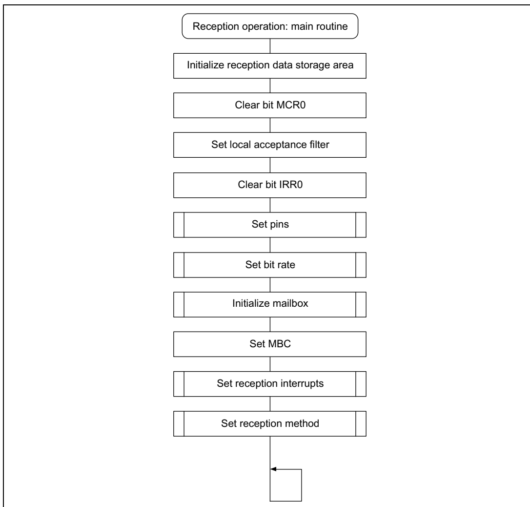
Figure 3.3 Reception Flowchart (1)
