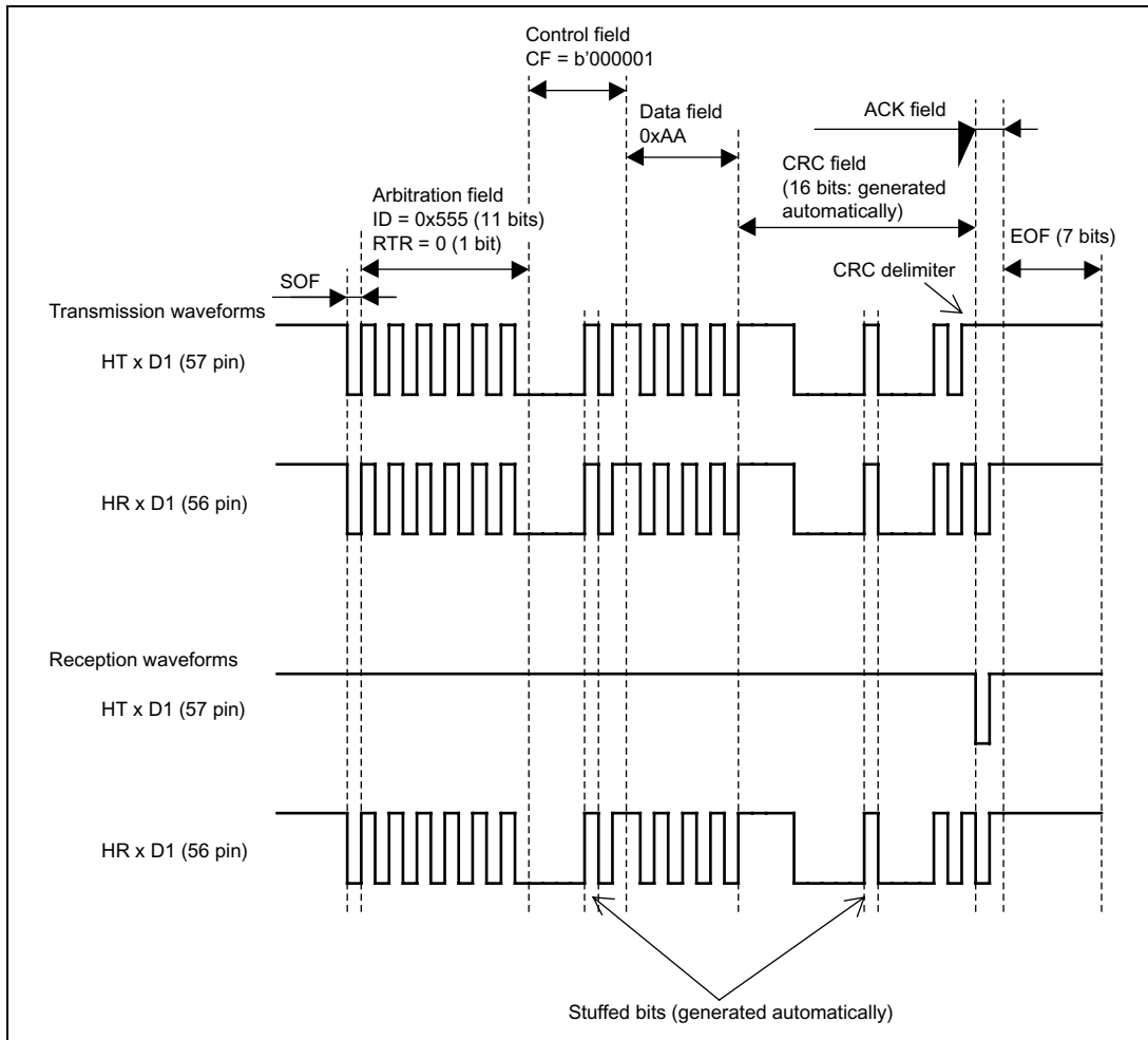
Figure 1.3 Operation Waveforms
