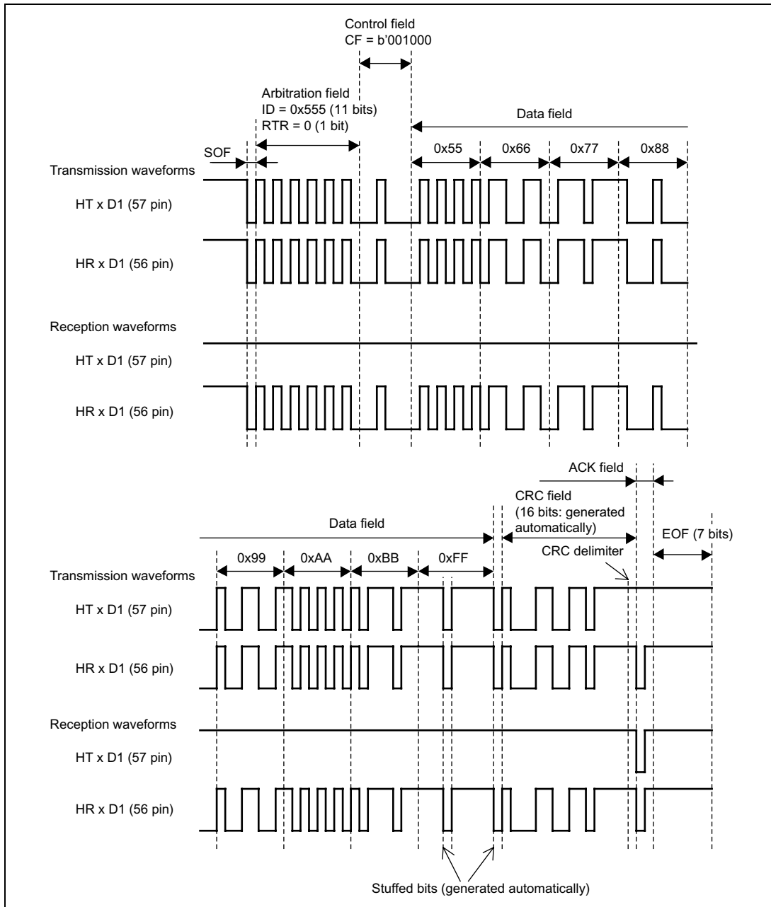
Figure 2.5 Operation Waveforms
