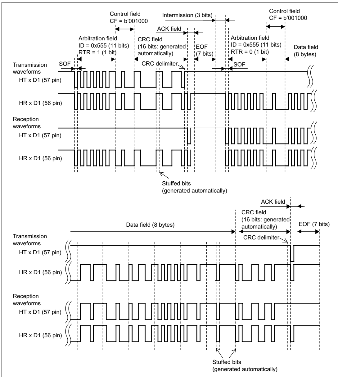
Figure 5.6 Operation Waveforms
