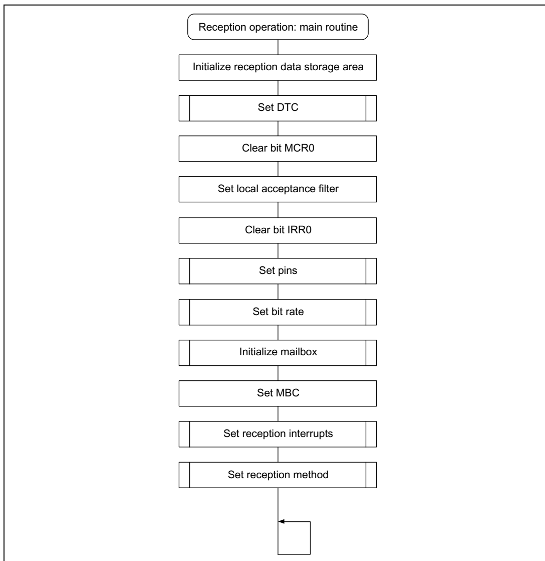
Figure 2.3 Reception Flowchart (1)
