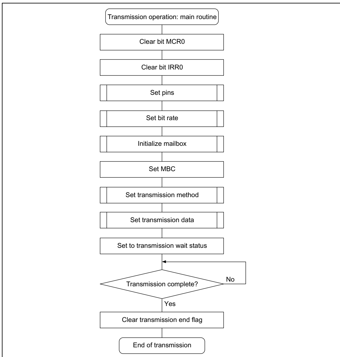
Figure 1.1 Transmission Flowchart
