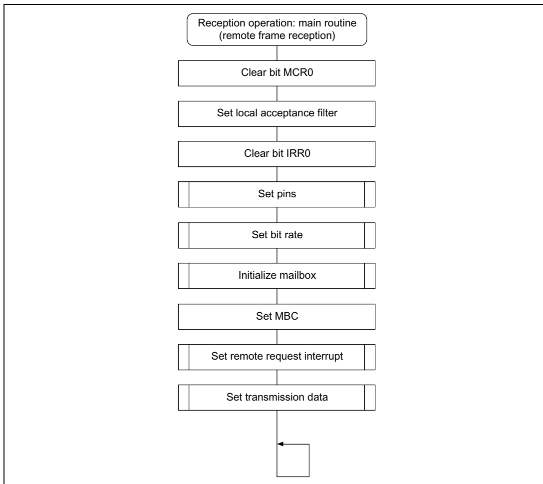
Figure 5.4 Reception Flowchart (1)
