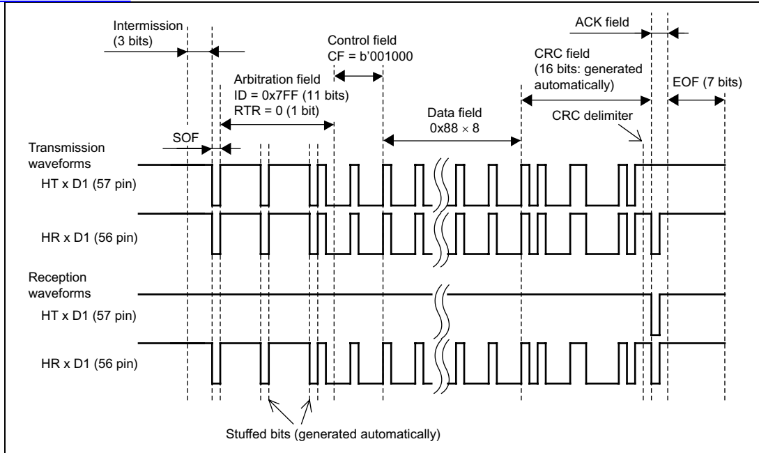
Figure 4.6 Operation Waveforms (End of Operation)
