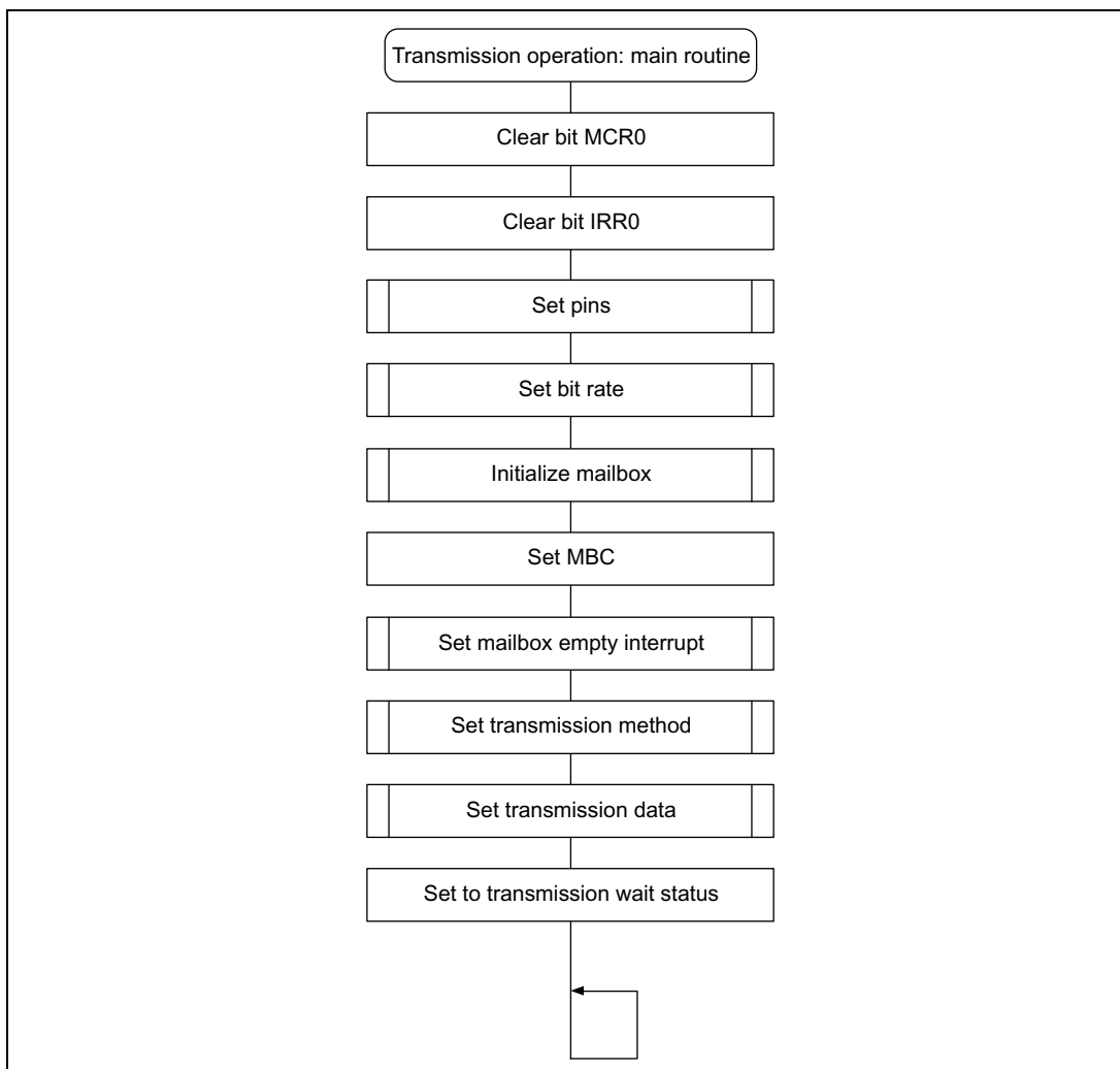
Figure 2.1 Transmission Flowchart (1)
