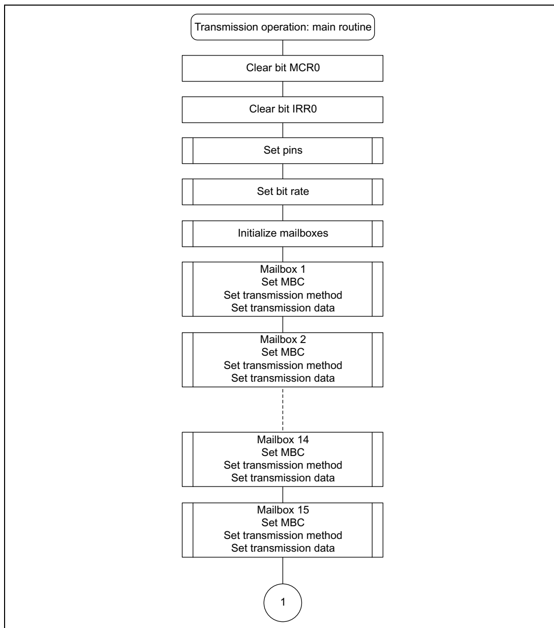
Figure 4.1 Transmission Flowchart (1)
