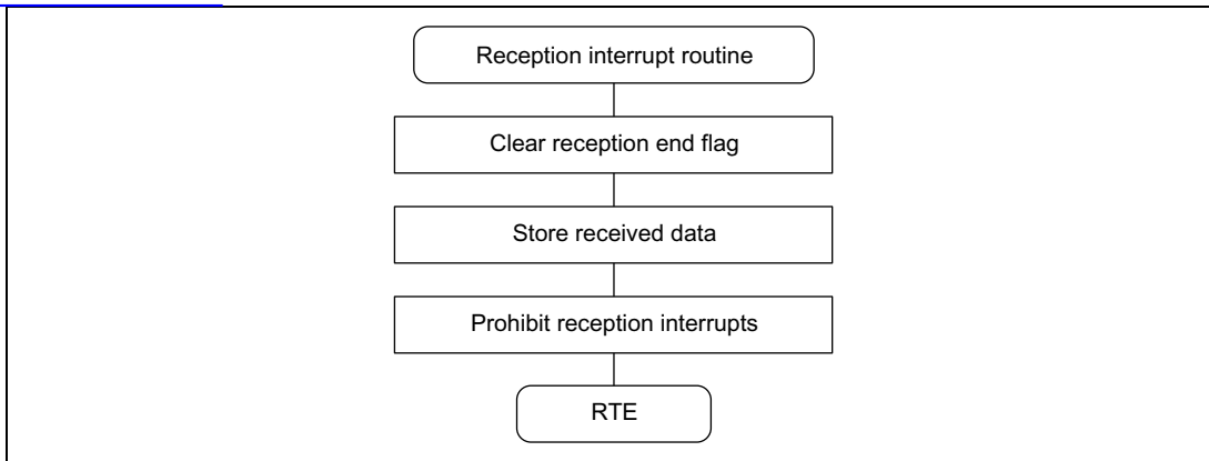
Figure 3.4 Reception Flowchart (2)
