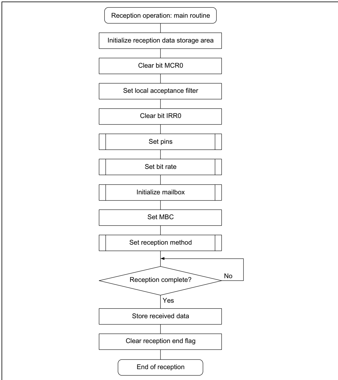
Figure 1.2 Reception Flowchart
