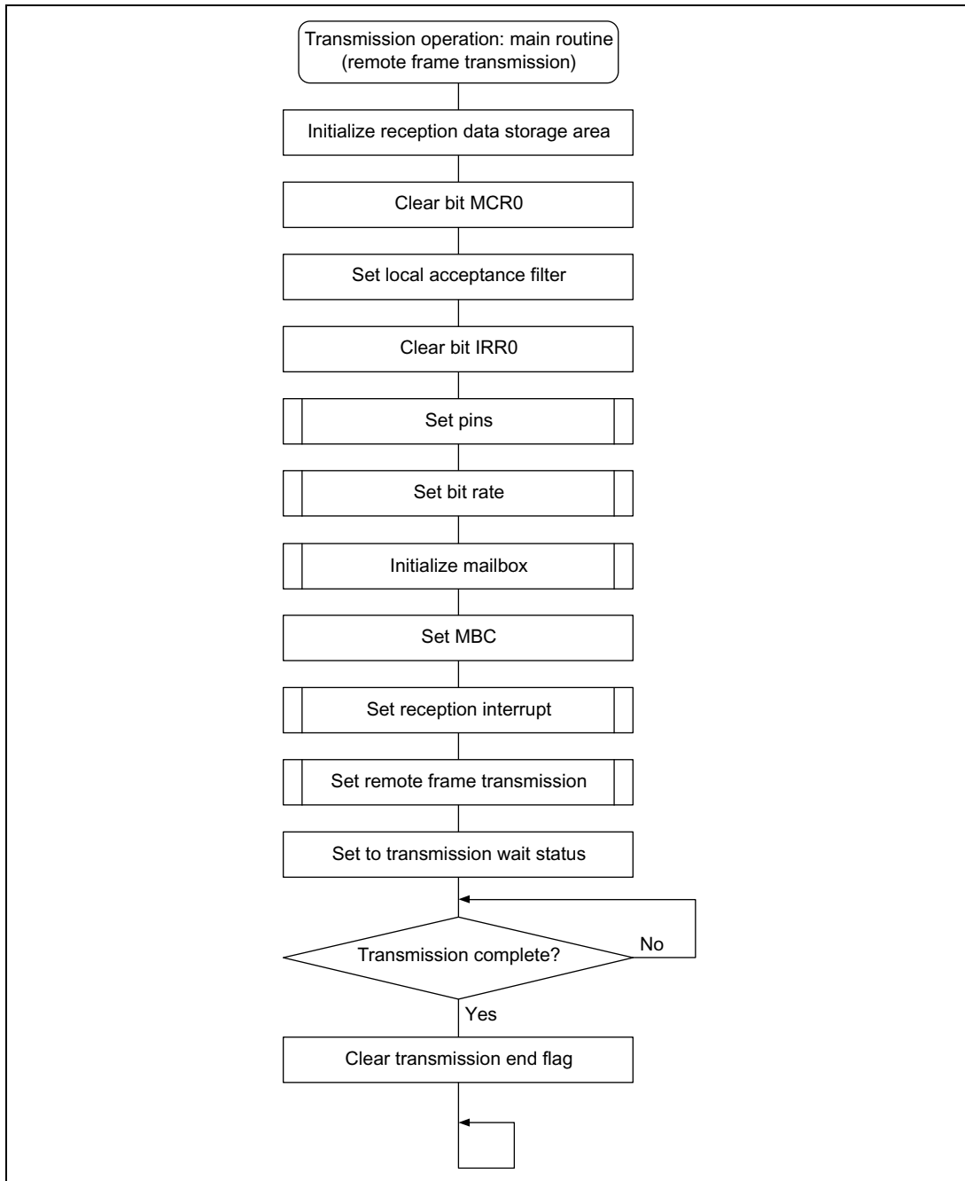
Figure 5.1 Transmission Flowchart (1)
