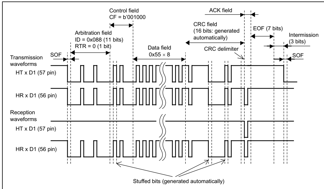
Figure 4.5 Operation Waveforms (Start of Operation)
