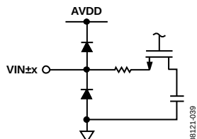
Figure 29. Equivalent Analog Input Circuit
