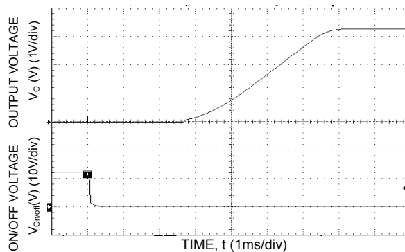
Figure 15. Typical Start-Up Using Remote On/Off with Low-ESR external capacitors ( 7 \times 150\ \mu\text{F} Polymer) ( V_{IN} = 12.0\text{Vdc} , V_o = 3.3\text{Vdc} , I_o = 3\text{A} , C_o = 1050\ \mu\text{F} ).
