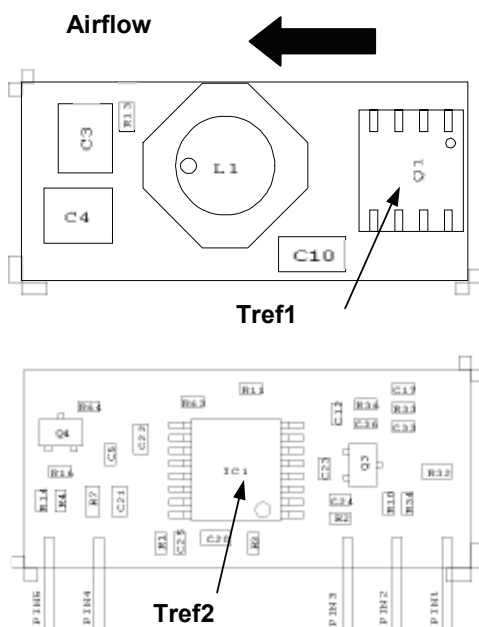
Figure 31. T_{ref} Temperature measurement location.
