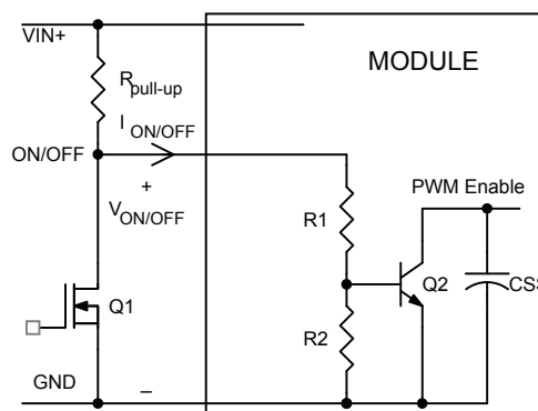
Figure 28. Circuit configuration for using negative logic On/Off.
