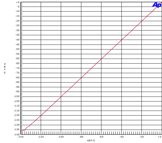
Figure 78. Linearity Error – 0 to -140 dBFS Input, 200 Hz Tone, 192 kHz:44.1 kHz
