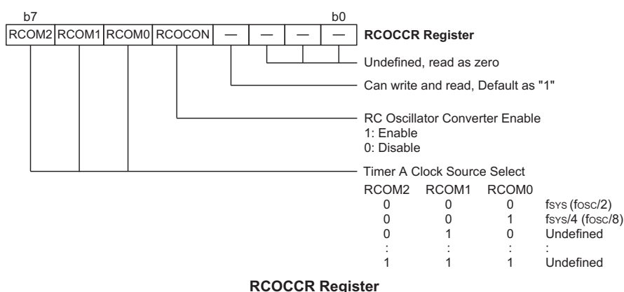
RCOCCR Register
