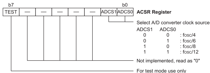
ACSR Register
