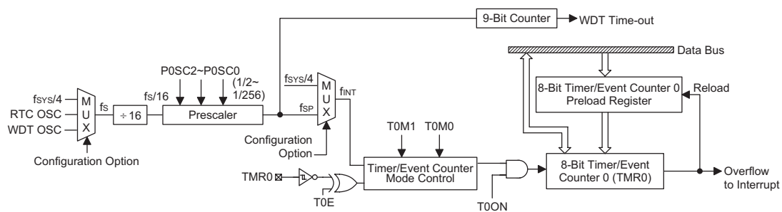
8-bit Timer/Event Counter 0 Structure
