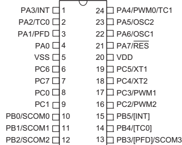
HT48R067 24 SKDIP-A/SOP-A/SSOP-A
