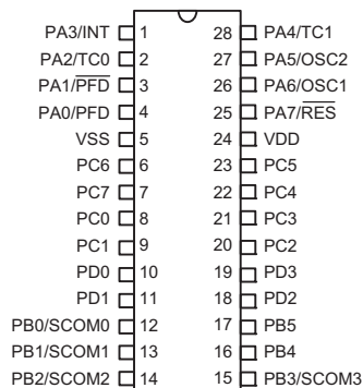
HT48R066 28 SKDIP-A/SOP-A/SSOP-A
