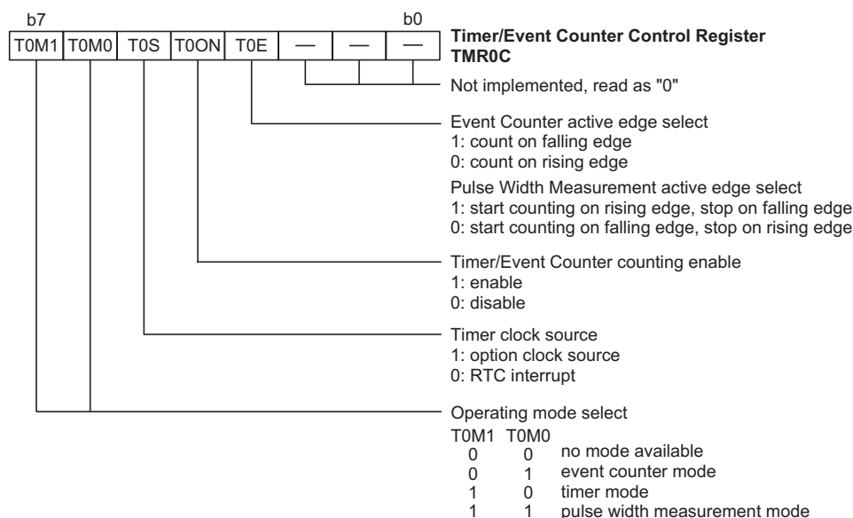
Timer/Event Counter 0 Control Register – TMR0C
