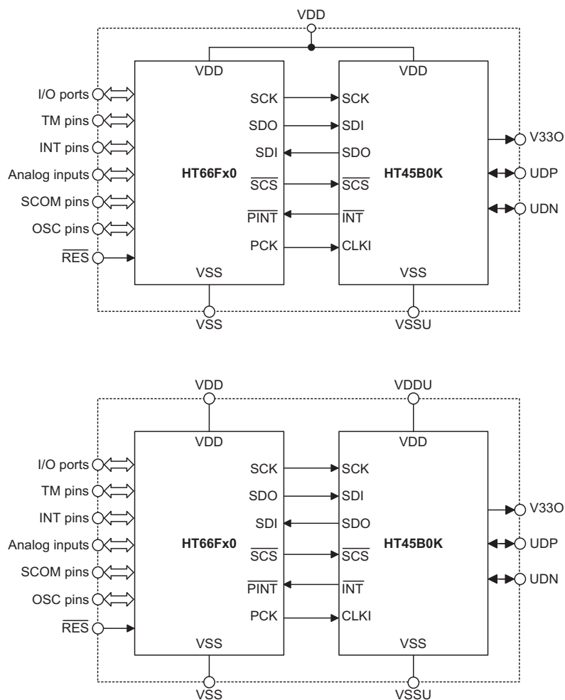
Internal Chip Interconnection Diagram
