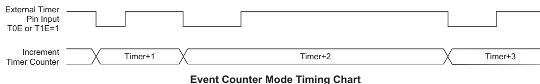
Event Counter Mode Timing Chart
