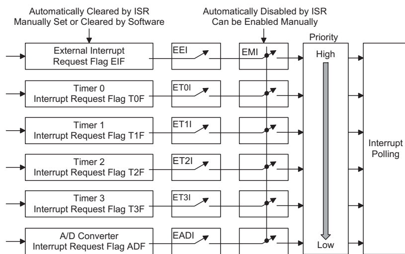
Interrupt Structure
