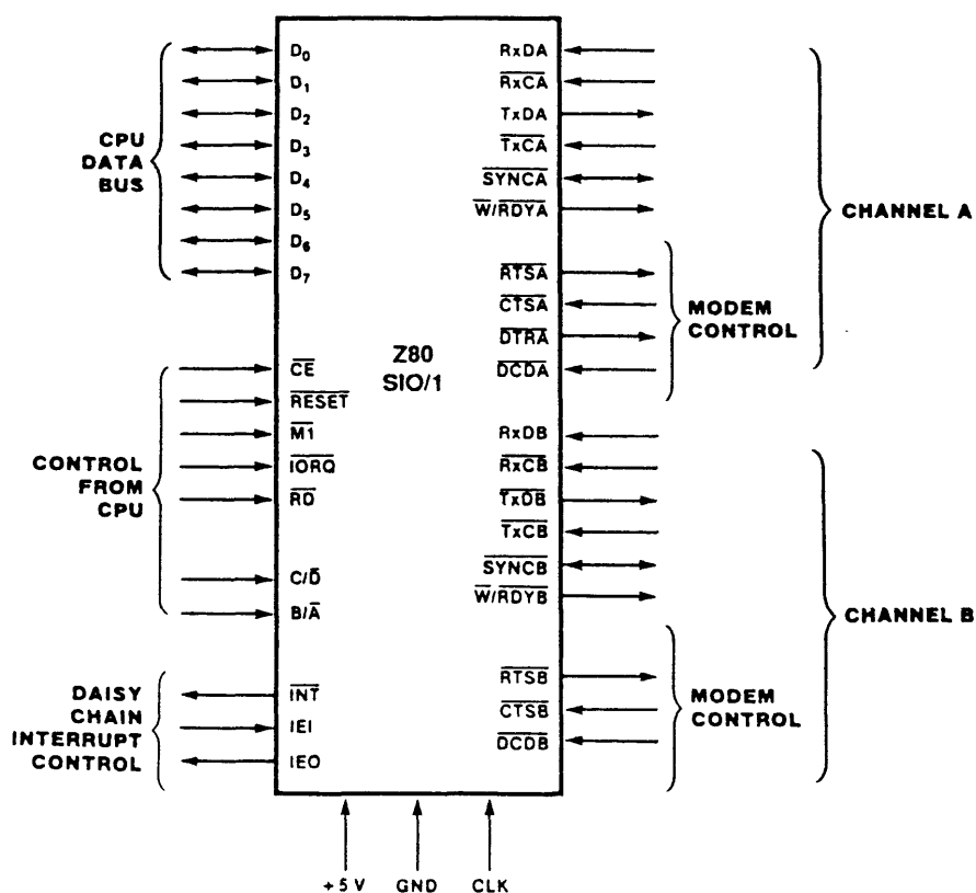
Figure 3. Pin Functions
