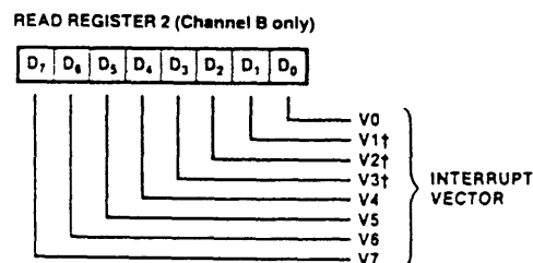
Figure 13. Read Register Bit Functions
