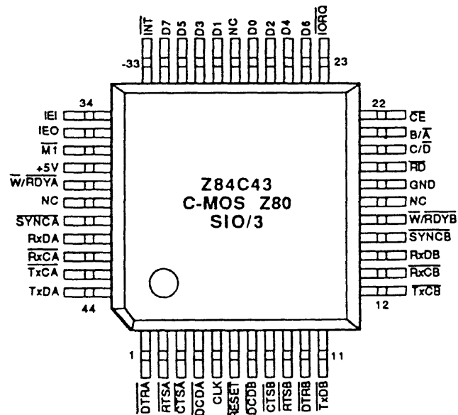
Figure 7b. 44-pin Quad Flat Pack Pin Assignments
