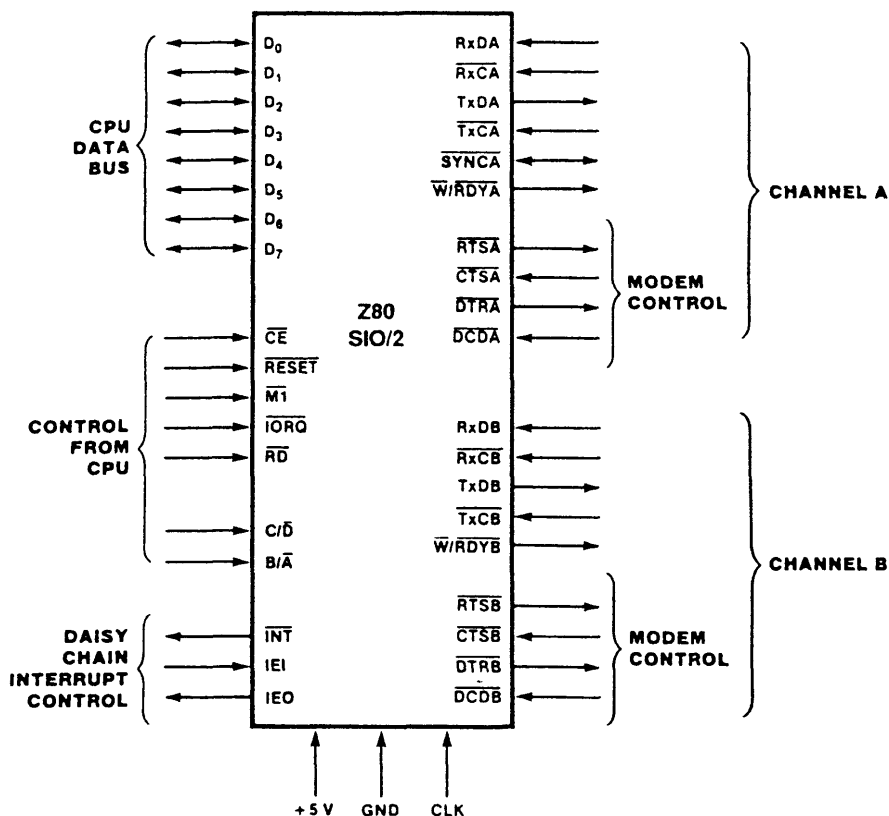
Figure 1. Pin Functions
