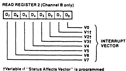
Figure 13. Read Register Bit Functions
