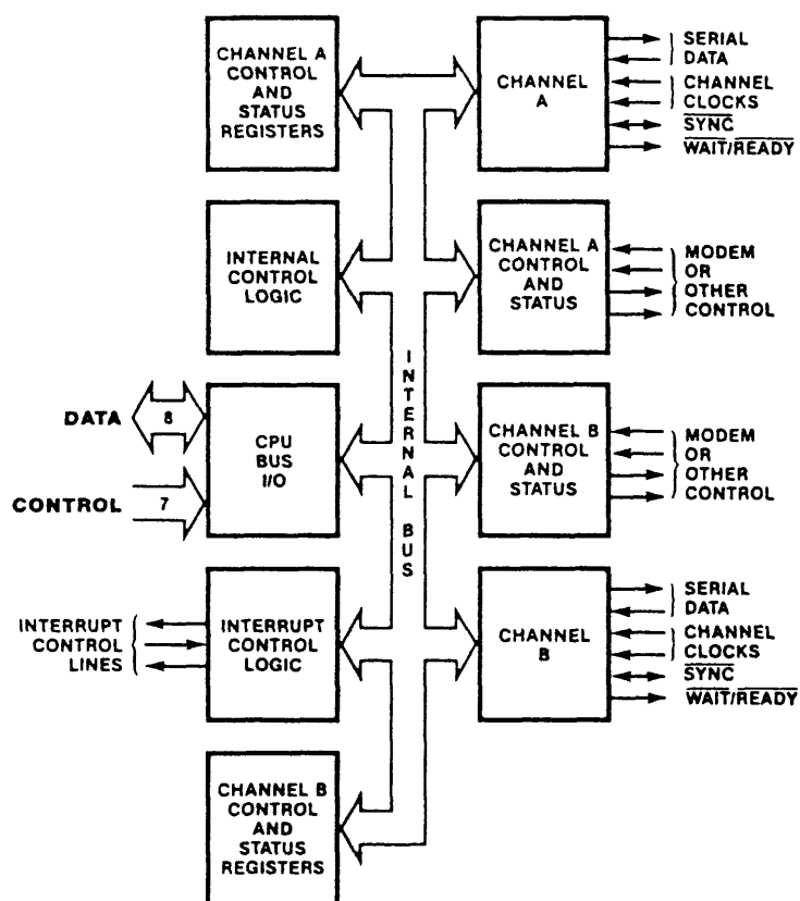
Figure 8. Block Diagram
