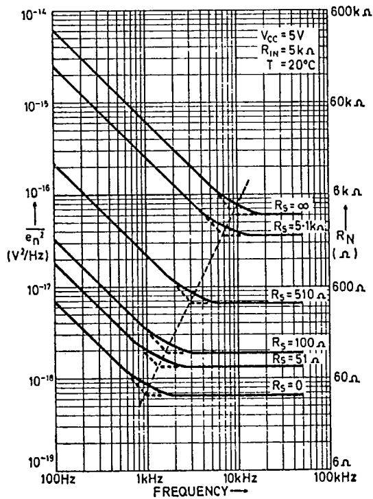
NOISE VOLTAGE
