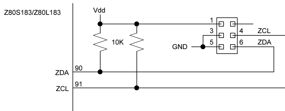
Figure 27. ZDI Connector on Target Board
