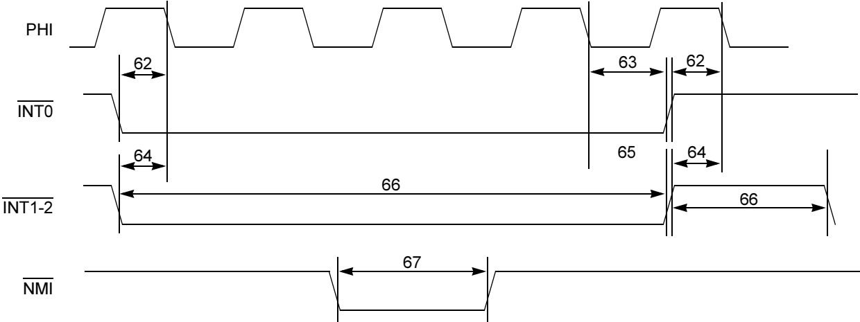
Figure 23. Interrupt Timing
