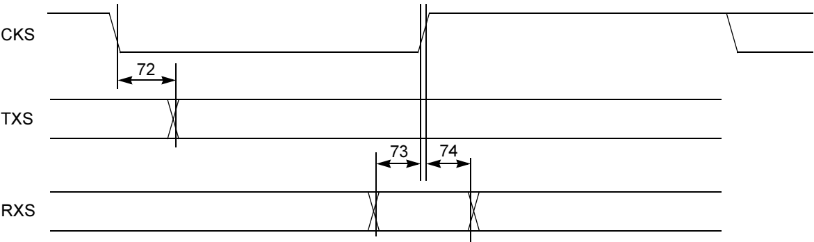
Figure 25. CSI/O Timing
