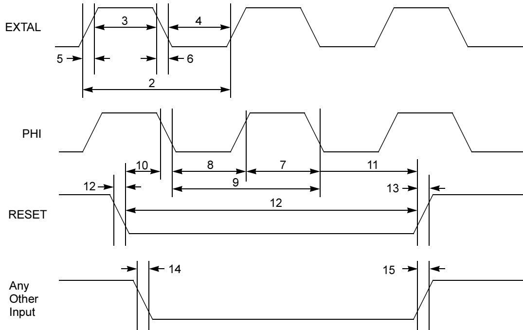
Figure 17. Basic Timing
