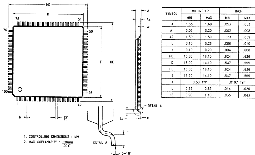
Figure 28. 100-Pin VQFP Package Diagram
