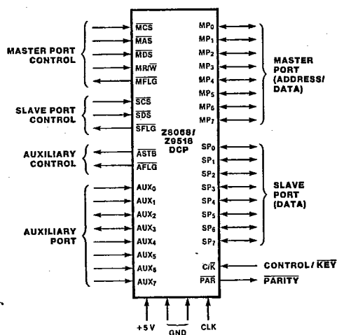
Figure 1. Pin Functions
