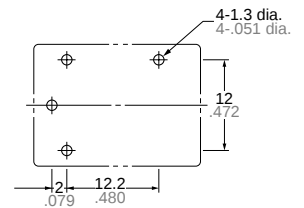
PC board pattern (Copper-side view)
