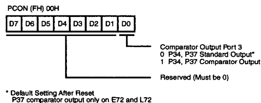
Figure 35. Port Configuration Register (PCON) (Write Only)
