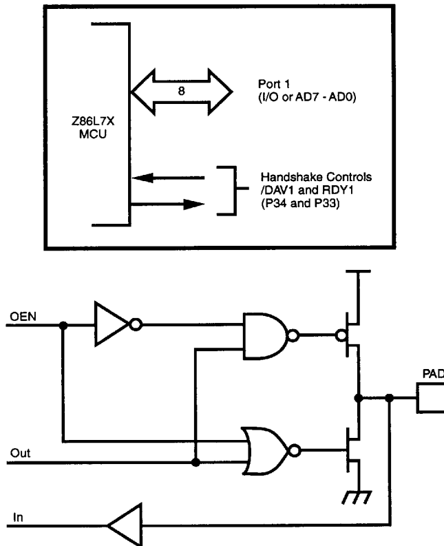
Figure 9 . Port 1 Configuration
