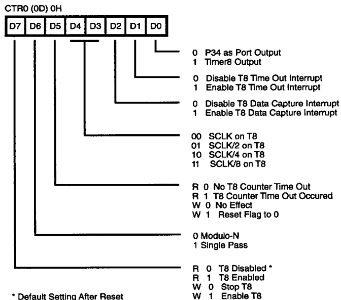
Figure 47. TC8 Control Register ((0D) 0H: Read/Write Accept Where Noted)
