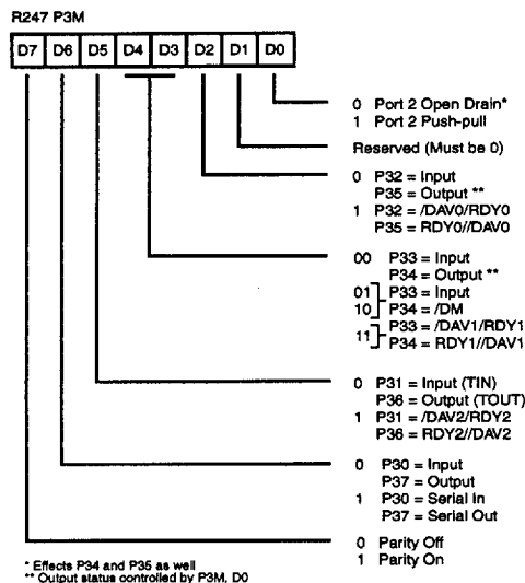
Figure 55. Port 3 Mode Register (F7H:Write Only)
