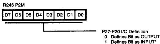
Figure 54. Port 2 Mode Register (F6H:Write Only)
