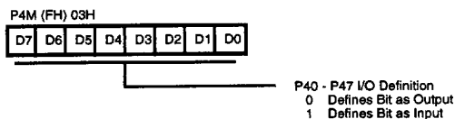
Figure 65. Port 4 Mode Register (F)03: (Write Only)
