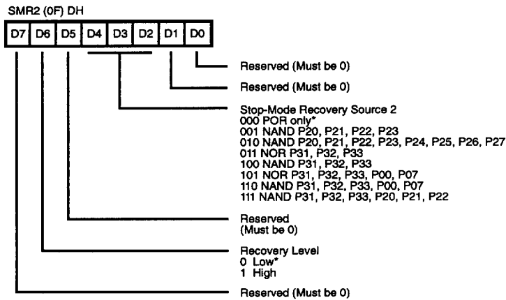
Figure 50. Stop-Mode Recovery Register (F)0BH: D6-D0 = Write Only, D7 = Read Only
