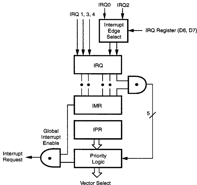
Figure 33. Interrupt Block Diagram
