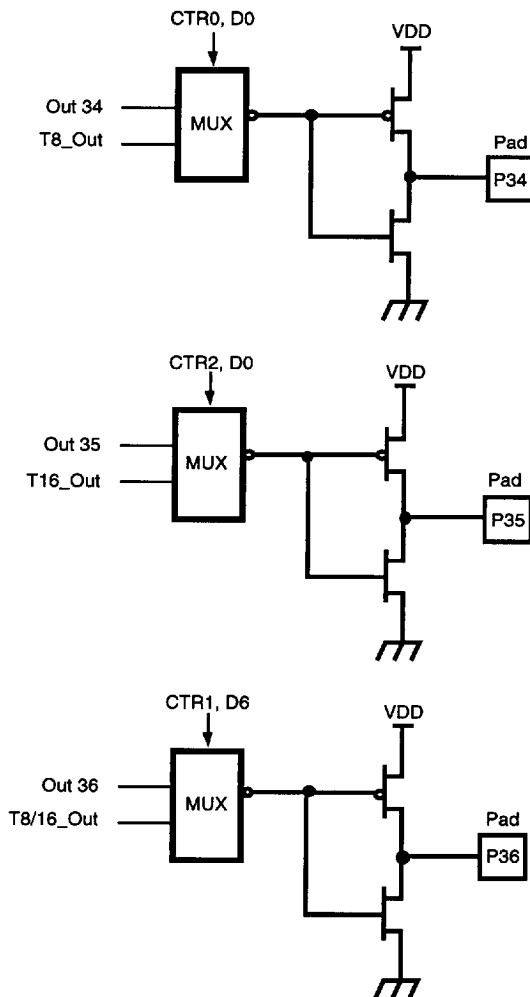
Figure 13. Port 3 Configuration
