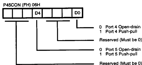
Figure 68. Port 4/5 Configuration Register (F)06: (Write Only)
