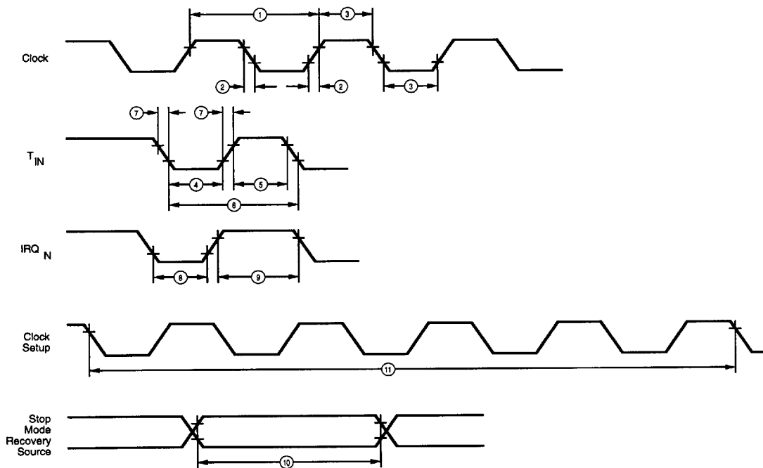
Figure 44. Additional Timing
