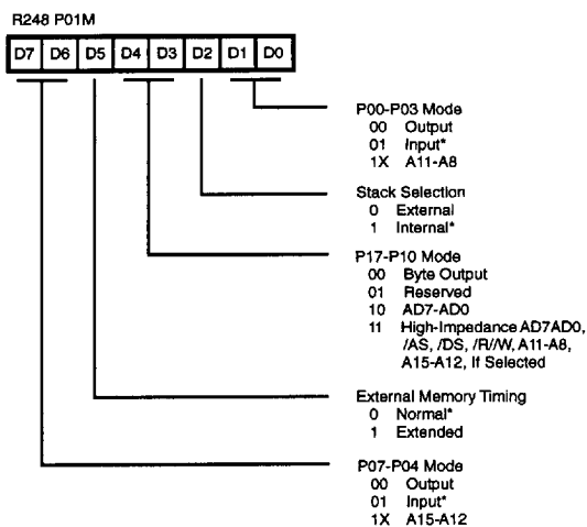
Figure 56. Port 0 and 1 Mode Register (F8H: Write Only)
