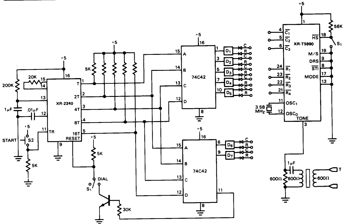
Figure 4. Typical Application Circuit for Auto Dialer Modem
