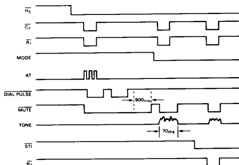
Figure 2. XR-T5990 Timing Diagram
