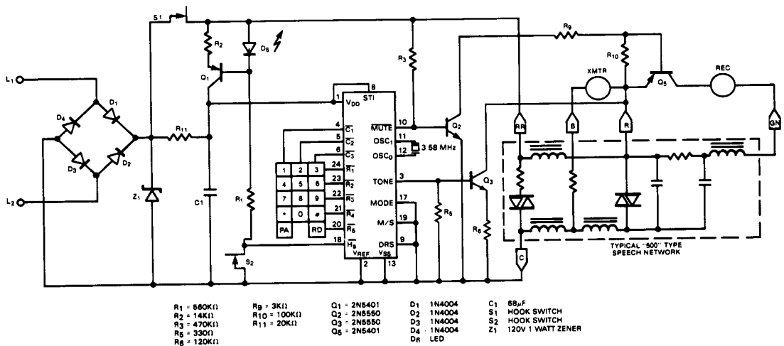
Figure 5. Typical Tone Dialing Application Circuit
