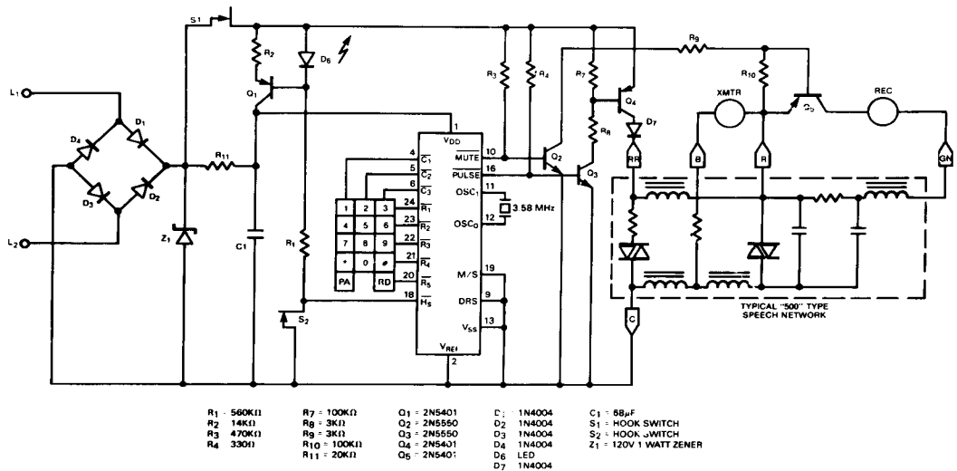
Figure 6. Typical Pulse Dialing Application Circuit
