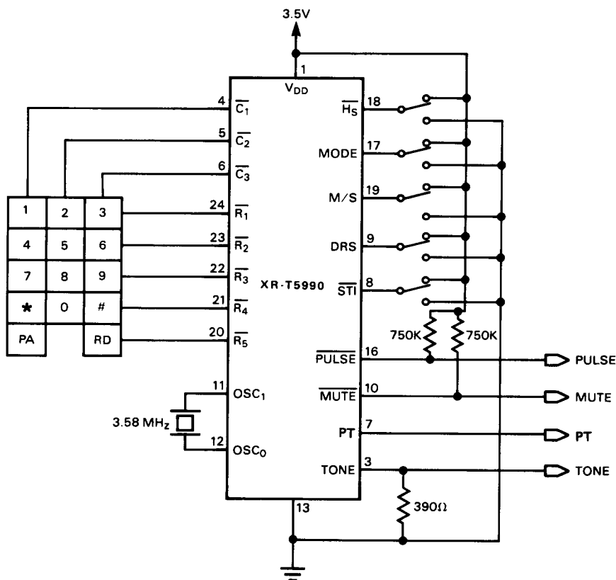
Figure 3. XR-T5990 Test Circuit
