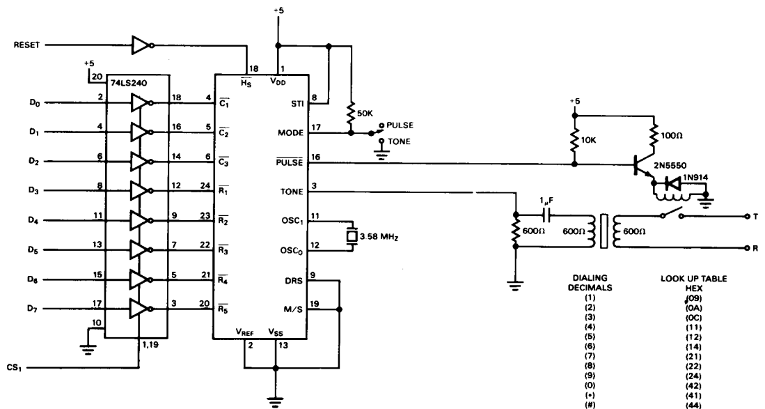
Figure 7. Typical Microprocessor Interface Circuit
