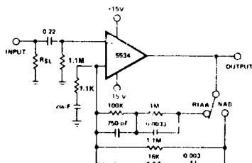
PREAMPLIFIER—RIAA/NAB COMPENSATION
