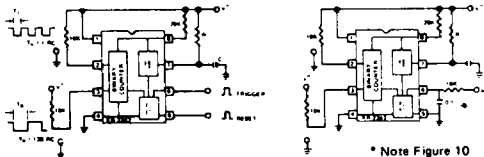
Figure 11. Astable Operation with External Trigger and Reset Controls
