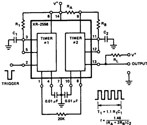
Figure 22. Keyed Oscillator
