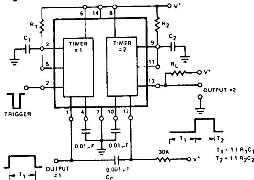
Figure 21. Sequential Timing
