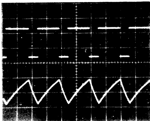
Figure 16. Astable Waveforms
