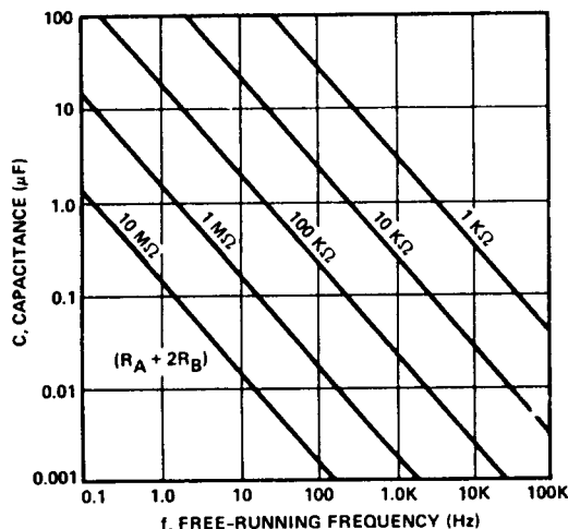
Figure 17. Free Running Frequency as a Function of External Timing Components
