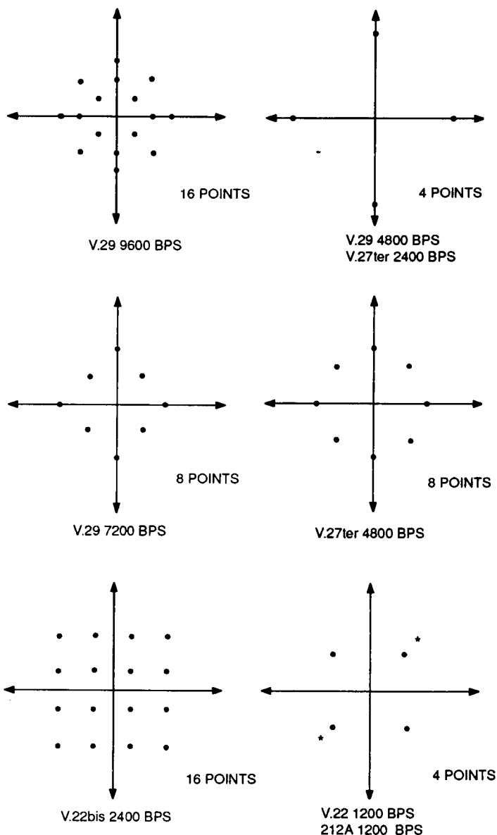
Figure 6. Signal Constellations
