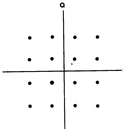
Figure 14. General Characteristics of 16 Point Constellation at 2400 BPS Q I
