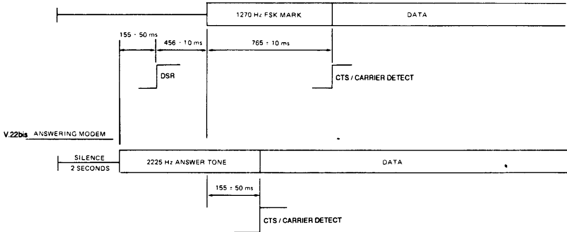
Figure 7. 103 Handshake Sequence at 300 BPS with 103 Modem
