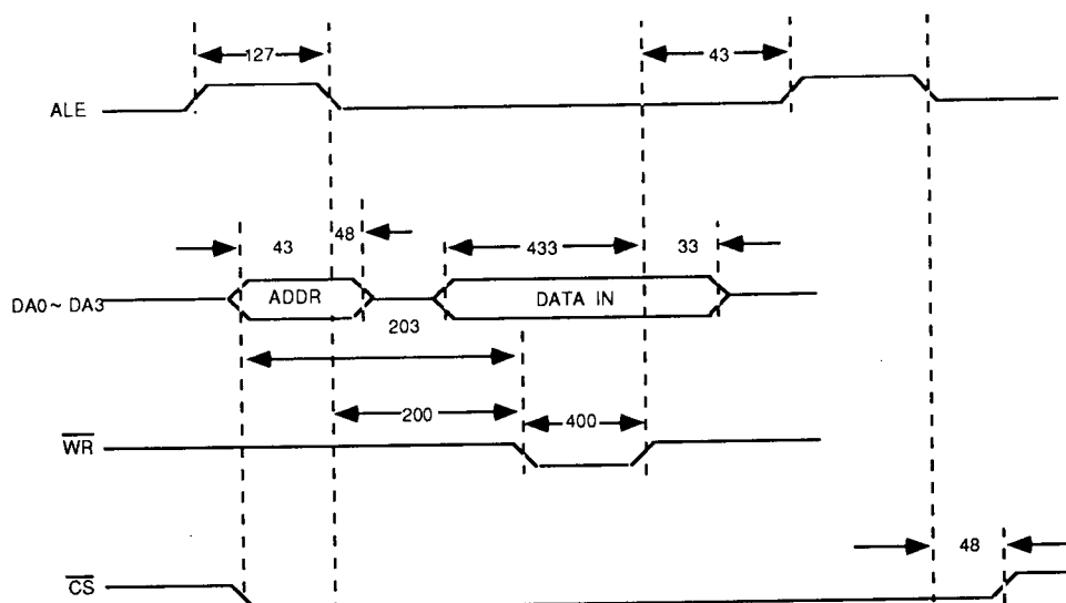
Write Cycle
