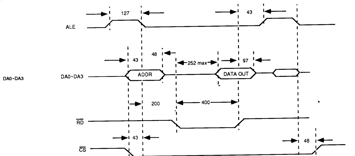
Read Cycle
